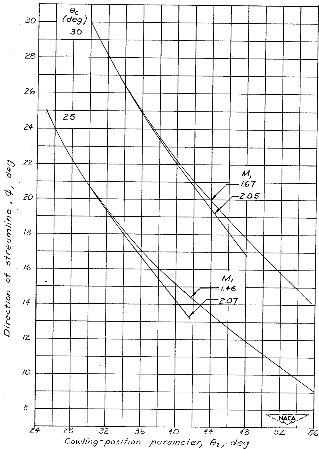
Figure 9.- Direction of the streamline for different Mach numbers and cone angles as a function of cowling-position parameter.
