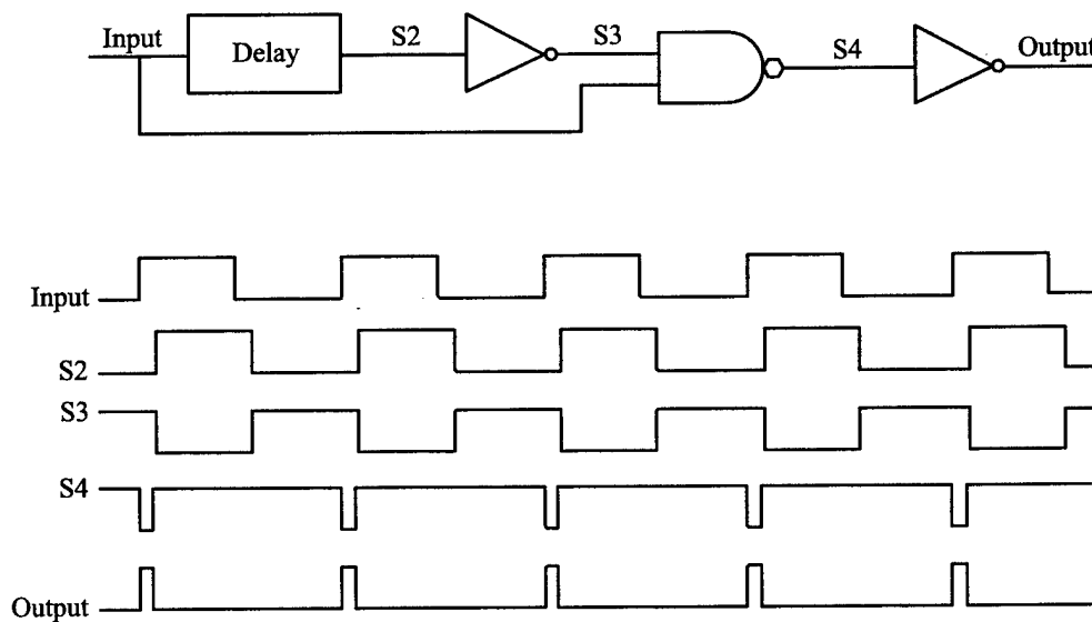
Figure 2.3-2. Block diagram of pulse amplifier rising edge detector.
