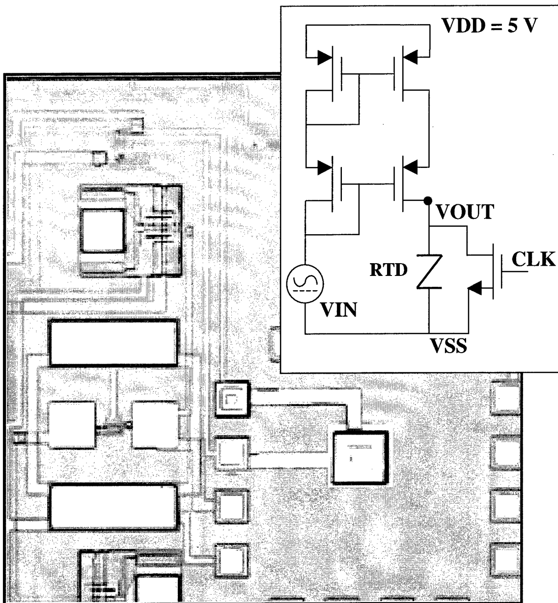
Figure 3. An Integrated RTD/CMOS Comparator. The RTD die measures 95 \times 95\text{ }\mu\text{m} , with a 16\text{ }\mu\text{m} diameter RTD. The circuit schematic is given in the inset.
