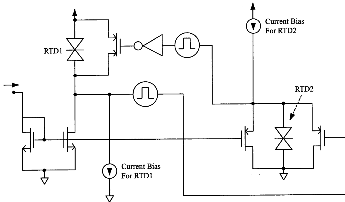
Figure 2.3-1. Schematic of the RTD/CMOS current mode pulse amplifier.
