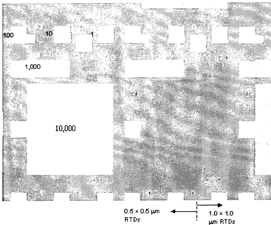
Figure 3.2-1. RTD arrays on die. Only the 0.5 μm and the 1.0 μm devices are illustrated. For all the device sizes, there are arrays of 1, 10, 100, 1000, and 10,000 RTDs.
