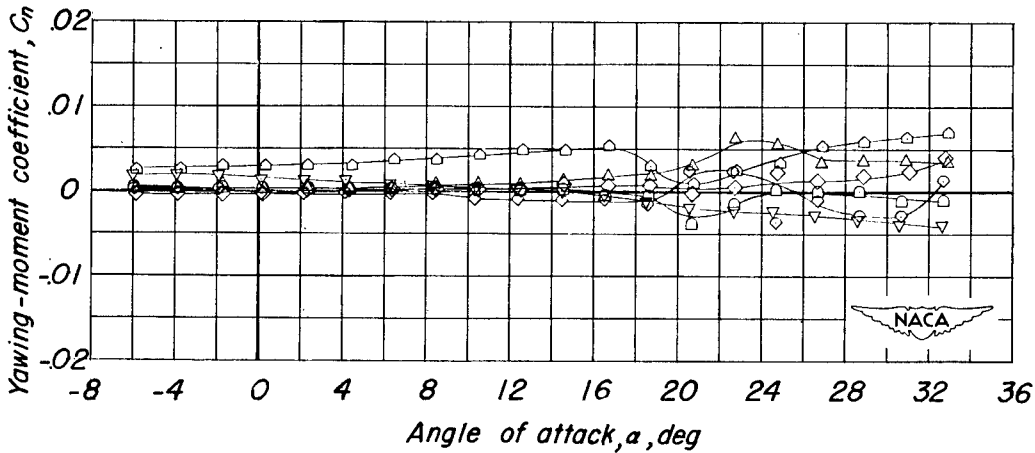
Figure 10.- Variation of the lateral control characteristics of the A = 1.13 wing with angle of attack. Inboard ailerons; \frac{b_a}{b/2} = 0.455 .
