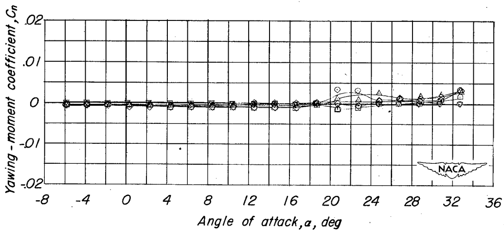
Figure 11.- Variation of the lateral control characteristics of the A = 1.13 wing with angle of attack. Inboard ailerons; \frac{b_a}{b/2} = 0.228 .
