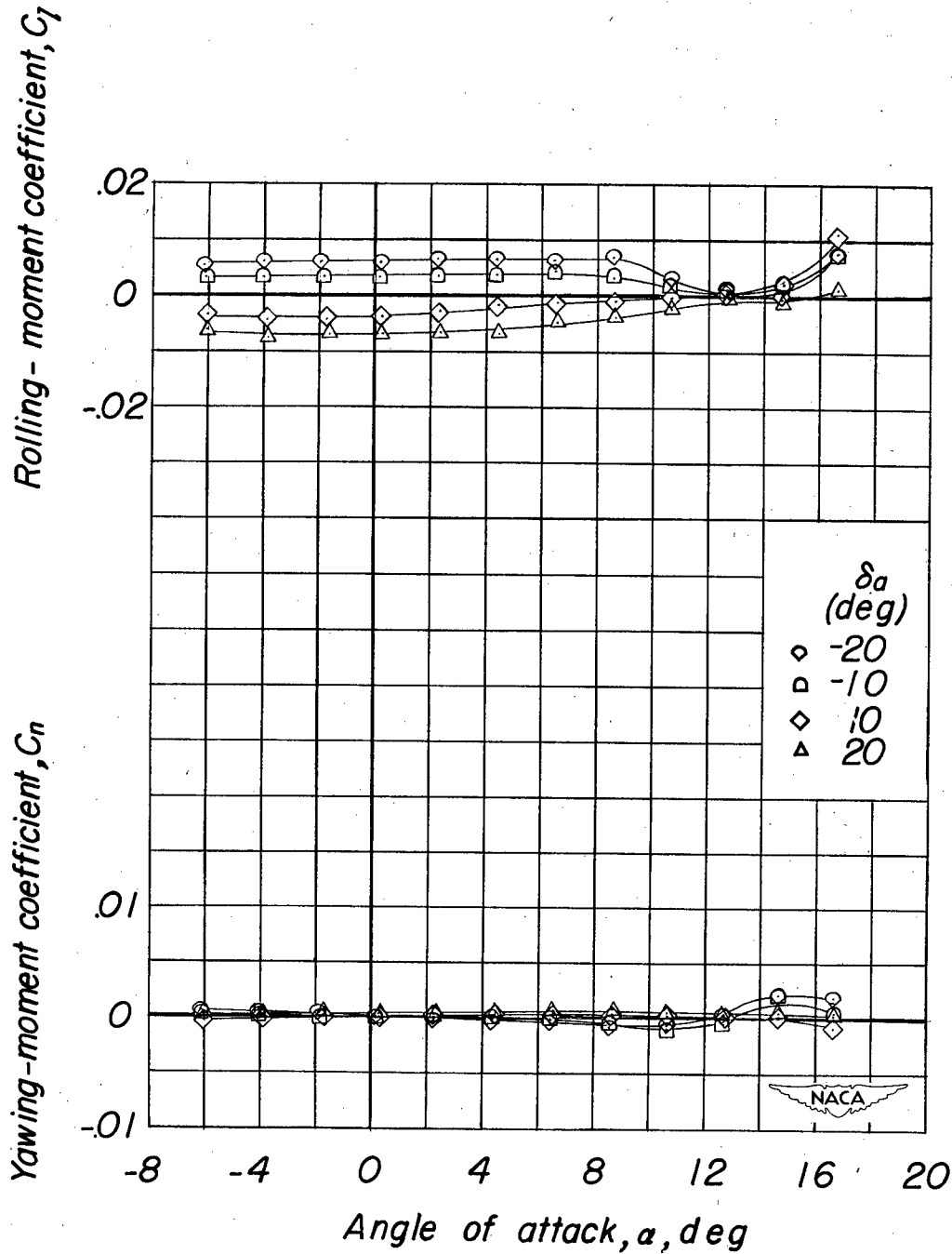
Figure 29.- Variation of the lateral control characteristics of the A = 6.13 wing with angle of attack. Inboard ailerons; \frac{b_a}{b/2} = 0.179 .
