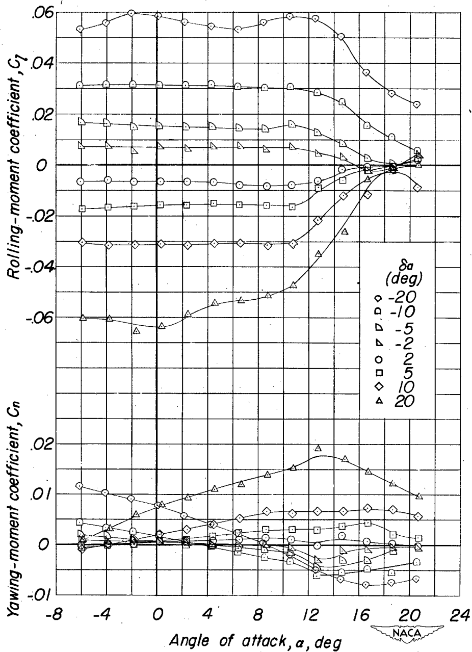
Figure 19.- Variation of the lateral control characteristics of the A = 4.13
