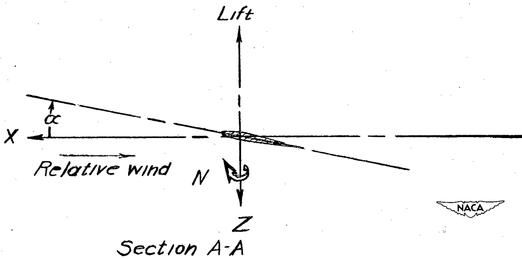
Figure 1.- System of stability axes. Positive values of forces, moments, and angles are indicated by arrows.
