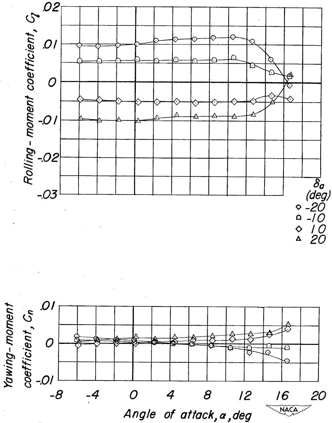
Figure 16.- Variation of the lateral control characteristics of the A = 2.13 wing with angle of attack. Inboard ailerons; \frac{b_a}{b/2} = 0.476 .
