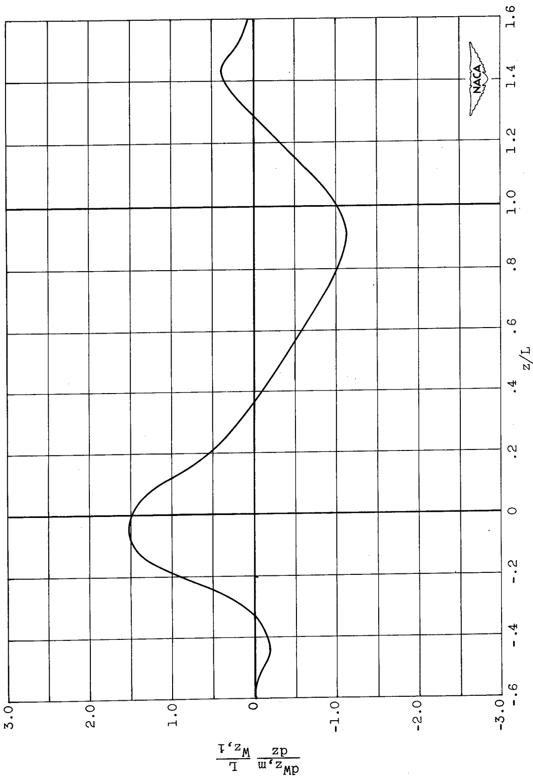
Figure 11. - Variation of total derivative of axial velocity on mean streamline with respect to axis for incompressible solution.
