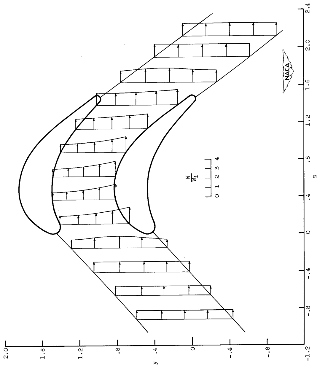
Figure 7. - Variation of magnitude of resultant velocity across channel for incompressible solution.
