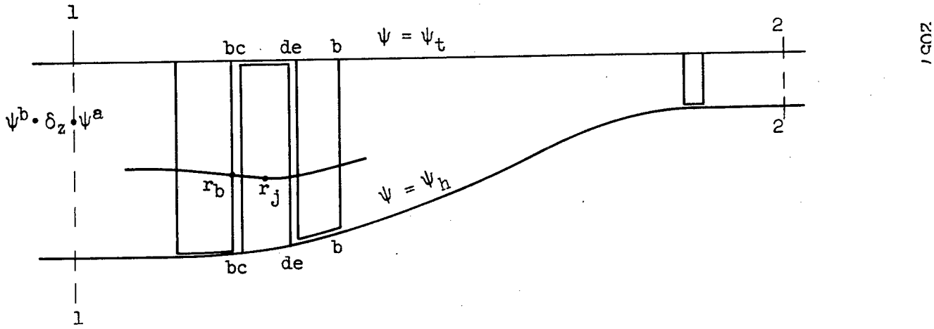
Figure 2. - Boundary conditions and station notation.
