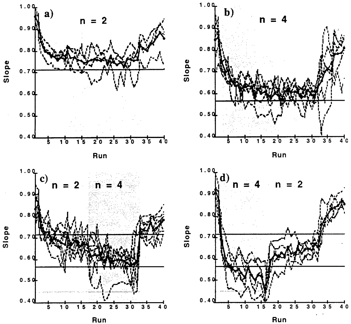
Figure 4. Individual subject and across-subject estimates of the best-fit slope as a function of run. Individual subjects given by dashed lines, across-subject averages by solid black line. Best-fit slope for the transformation(s) employed are shown by horizontal lines: pink is used to show the best-fit line for the n = 2 transformation, blue for the n = 4 transformation. The pink- and blue-shaded areas show which runs used the n = 2 and n = 4 transformation, respectively. a) n = 2 experiment, b) n = 4 experiment, c) n = 2 then n = 4 experiment, d) n = 4 then n = 2 experiment.
