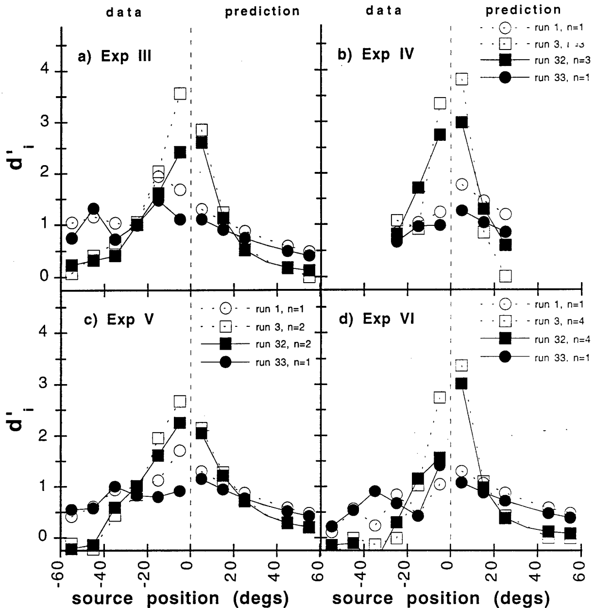
Figure 3. Actual and predicted d'_i as a function of position. Left side of each panel shows experimental results (averaged assuming data are left-right mirror symmetric). Right side of each panel gives predictions from the model for positions right of center. The dotted line separates the experimental data from the predicted results. Closeness of predictions is measured by the degree to which each panel is mirror symmetric. Again, the model predicts results quite closely. Model parameters were identical to the values used to predict total sensitivity (Figure 1) and bias (Figure 2).
