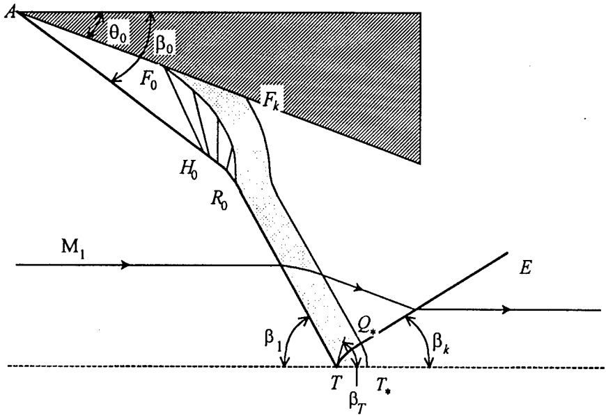
Fig. 3. Reflection of an oblique shock wave with the relaxation zone.
