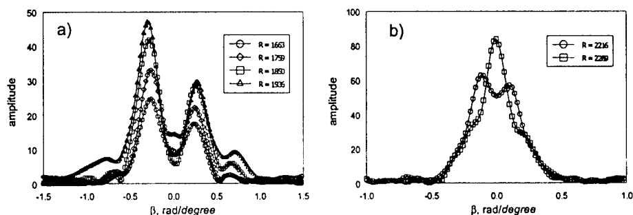
Figure 5. Transversal wave spectra of disturbance amplitude for first (a) and second (b) mode disturbances.
