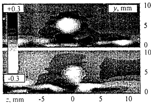
Figure 4. Contours of u(y,z)/U_0 at x=500 mm. Top: periodical, bottom: pulse excitation. Time instants are indicated on Fig. 3 by triangles
