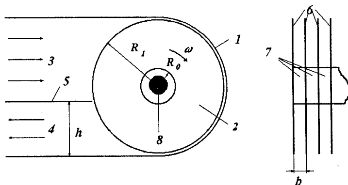
Fig. 1. 1 – body; 2 – rotor; 3 – input channel; 4 – output channel; 5 – separating partition; 6 – aluminium disks; 7 – separating rings; 8 – ohmic heater.
