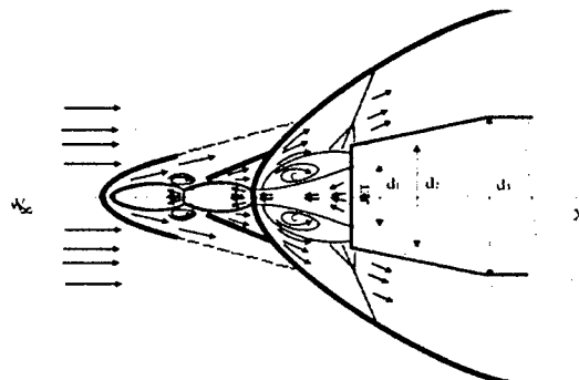
Fig. 3. Scheme of flow around the body with an upstream jet
