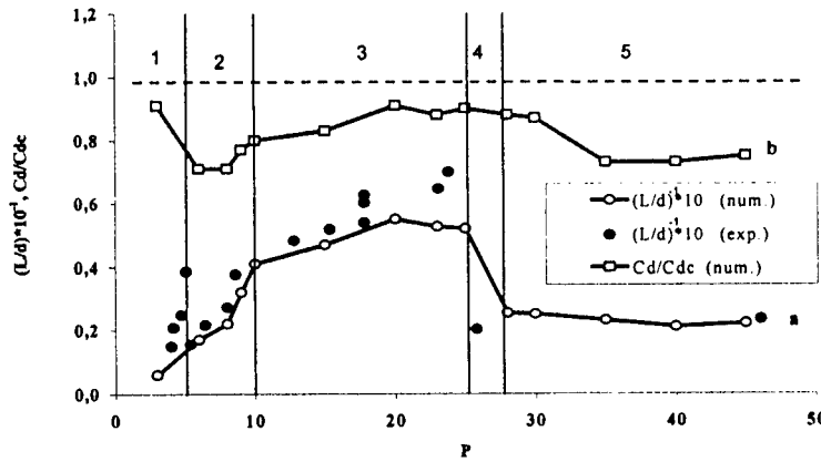
Fig. 1. Dependence of the length of jet penetration on pressure ratio (a), Dependence of the drag on pressure ratio (b).
