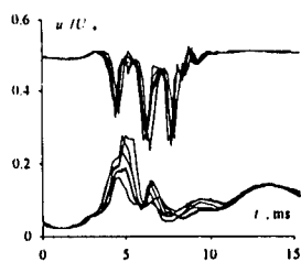
Figure 7. Not averaged time traces u_i(t)/U_0 (6 instants) at x=500 mm (3-spike stage). Top: y=4.5 mm, bottom: y=0.2 mm.
