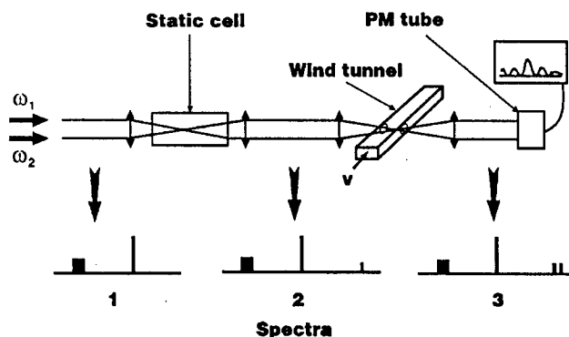
Fig. 4. Schematic diagram for CARS velocity measurement in a hypersonic flow.
