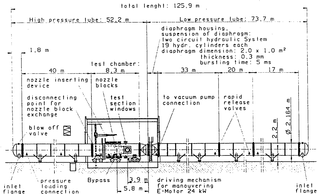
Details of Test Section (schematic)
