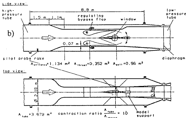
Fig. 2.1 a) The "shock wind tunnel" (SWK), total view; b) Principal construction and main dimensions of test section and corresponding scaled versions (schematic) used for calibration and comparative measurements
