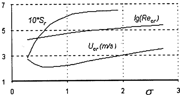
Fig. 2. The critical parameters: U_{cr} , \lg Re_{cr} and S_r for the Hopf bifurcation vs. the mass ratio \sigma for the strip's length l = 0.1-1.0 \text{ m} .
