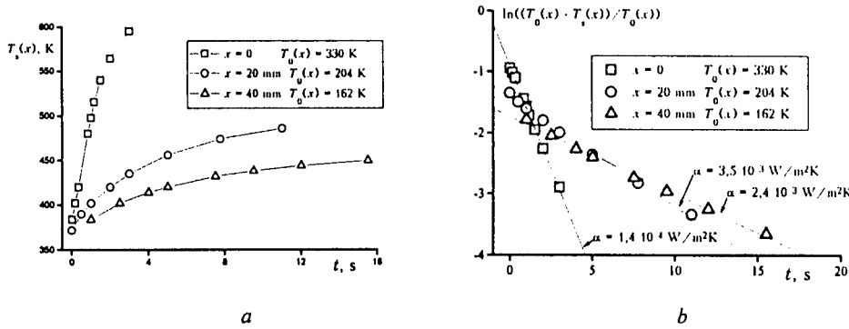
Fig. 2. Dependence of temperature on time for the flow of a plane supersonic isobaric air jet. p_0 = 1,45 \text{ MPa} , T_0^* = 330 \text{ K} , h^* = 3 \text{ mm} is the thickness of the jet on the nozzle edge, z_0 = 15 \text{ mm} .
