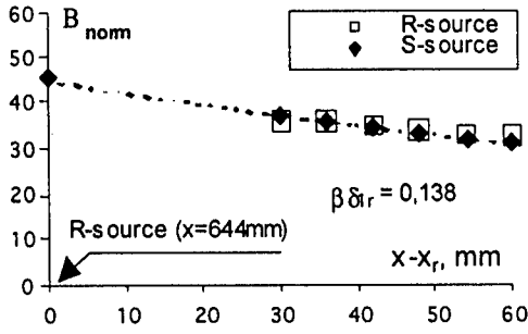
Fig. 4. Method of initial amplitudes determination.
