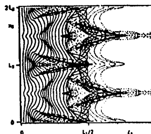
Fig. 9. Staggered and aligned in rows \Lambda -structures in channel flow. DNS [20, 21].
