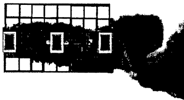
Fig. 3. Smoke-flow visualization (three beams, Sh=0.095 , A/H=0 ).
