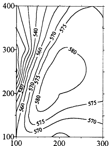
Fig. 6. Isolines of velocity of aluminum particles d_p = 10 \mu\text{m} at impact on the surface of an obstacle. z_0 = 15 \text{ mm} , T_0 = 470 \text{ K} , p_0 = 1.5 \text{ MPa} . Abscissa is 100h , mm, ordinate is L , mm. Numbers on the curves denote values of impact velocity, m/s.
