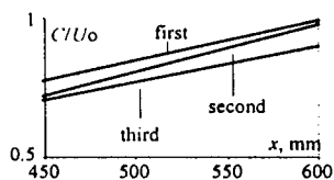
Figure 6. Downstream speeds of the first 3 ring-like vortices.
