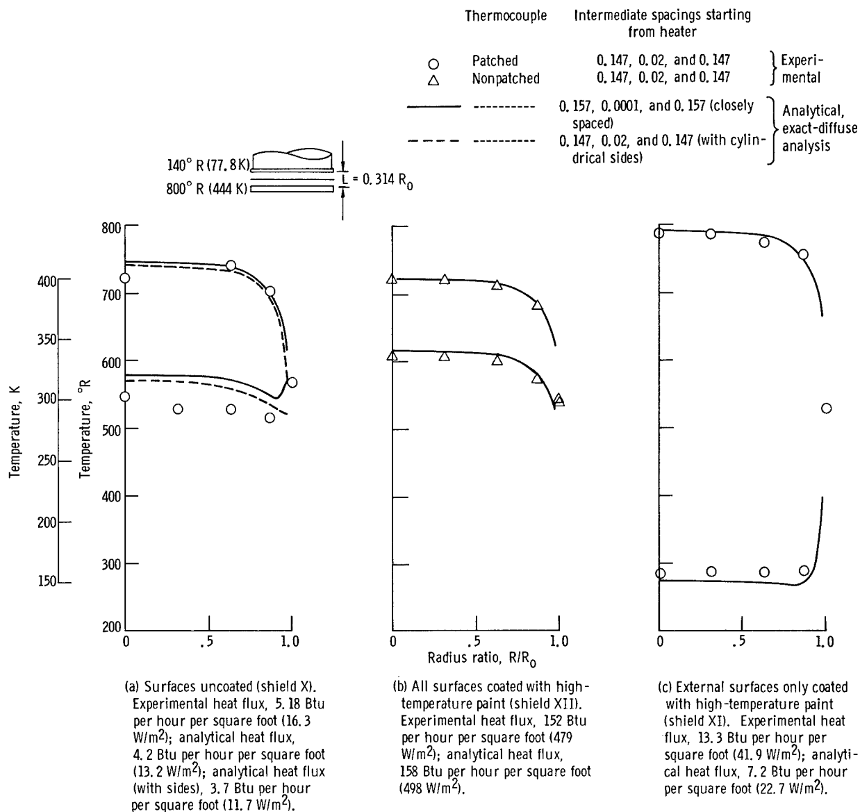
Figure 23. - Temperature profiles for various surface properties on double-sheeted shields.
