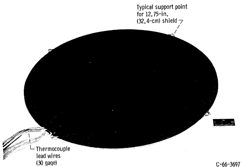
Figure 3. - Typical construction and instrumentation used for relatively thick copper, stainless-steel, and aluminum shadow shields (shields I, II, III, and IV).
