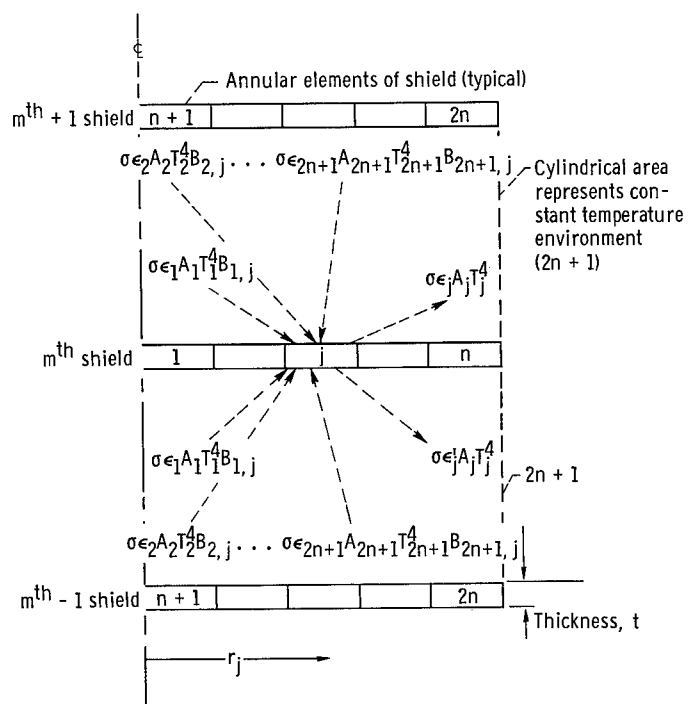
Figure 35. - Sketch showing radiant heat transferred to annular elemental area of shield.
