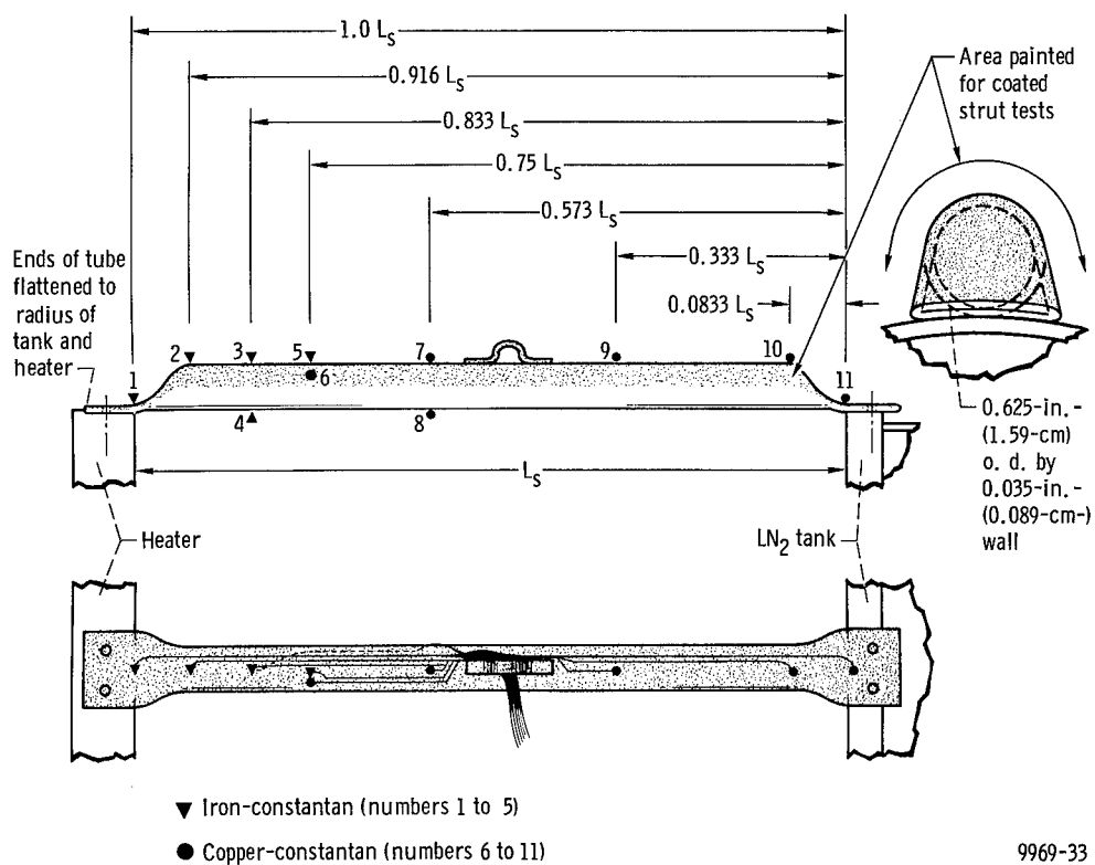
Figure 7. - Schematic diagram of support tubes and location of 30-gage thermocouples.
