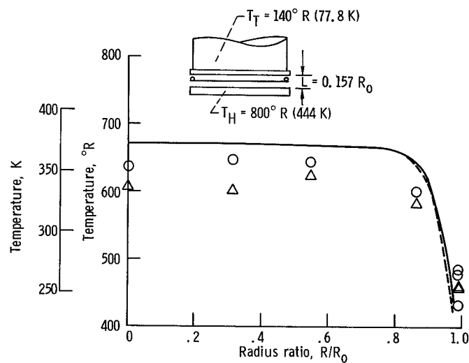
Figure 22. - Effect of thermocouple installation technique on local shield temperatures (shield IX). Analytical results assume shield is divided into 10 equal-area nodes and temperatures are plotted at mean area of each node. Heat flux (experimental), 10.4 Btu per hour per square foot (32.8 W/m 2 ).
