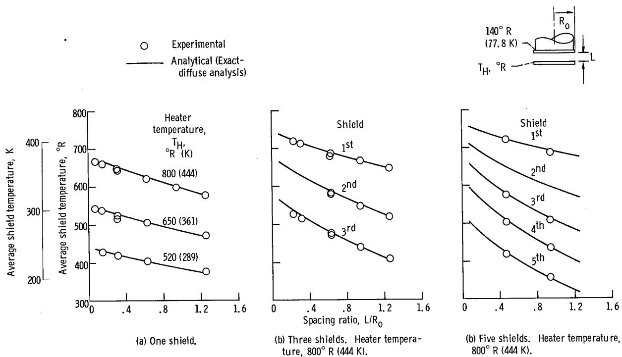
Figure 16. - Average shield temperatures for high-conducting, high-emissivity shield configurations (shield I).
