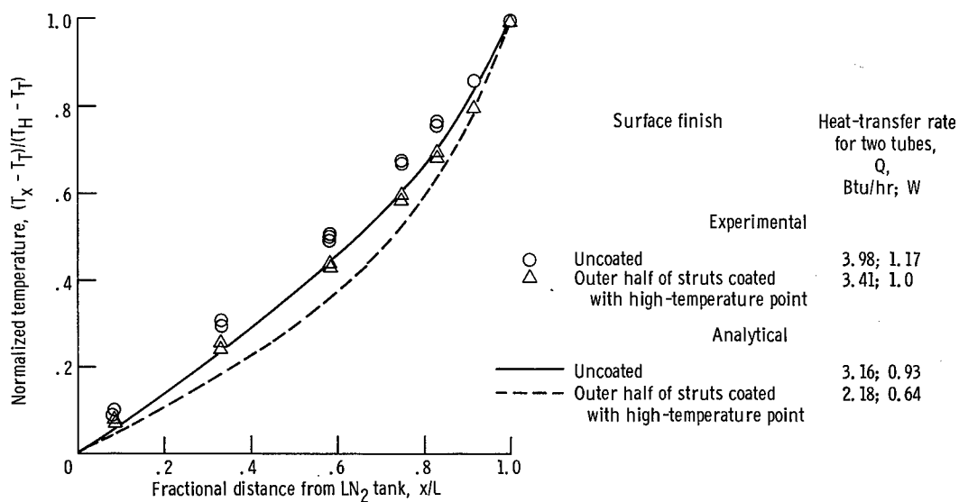
Figure 24. - Effect of external emissivity on temperature profile of 12-inch-long (30.5-cm-long) structural tube. Radiant heat transfer from shields < 0.01 Btu/hr (0.00293 W).
