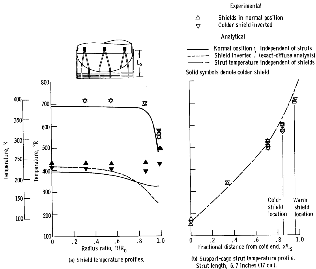
Figure 31. - Shield and support-cage temperature profiles for pinned shields (shield IX). L/R_0 = 0.192 .
