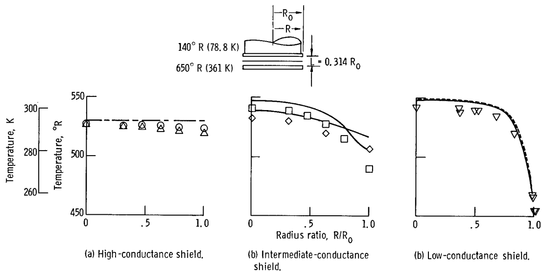
Figure 19. - Effect of lateral conductance on shield temperature profile and heat-transfer rate for single shield.
