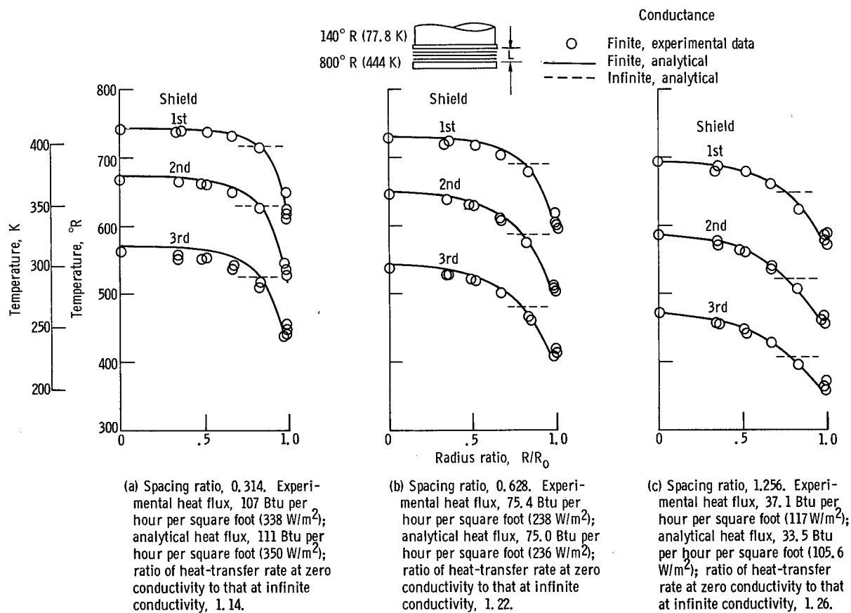
Figure 20. - Effect of spacing ratio on temperature profiles of three low-conductance shields (shield VI).
