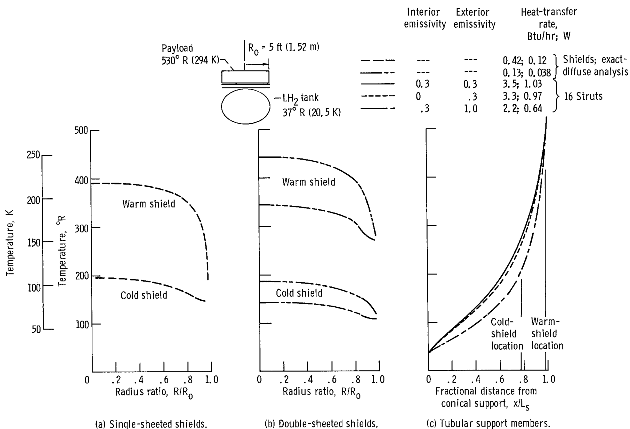
Figure 33. - Temperature profiles and heat-transfer rates for hypothetical shadow shield system. Payload, tank, and shield emissivity, 0.03; support ring emissivity, 0.3; lateral conductance, 0; spacing ratio, 0.192.
