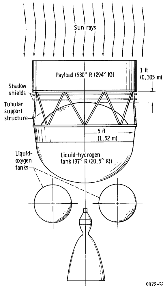
Figure 26. - Schematic of hypothetical hydrogen-oxygen upper stage. Structural details of vehicle below hydrogen tank are omitted for clarity.
