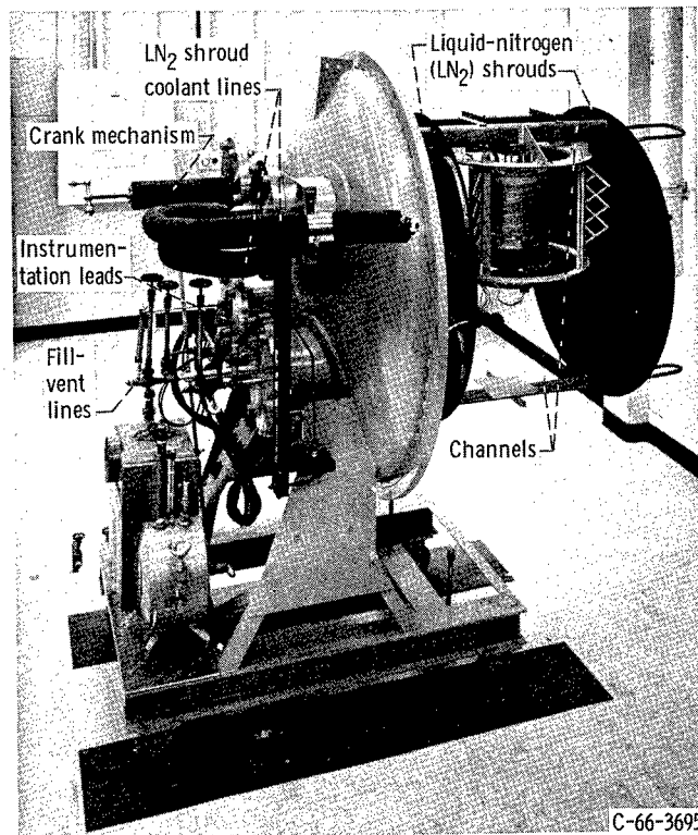
Figure 2. - Overall view of experimental apparatus connected to vacuum chamber door.
