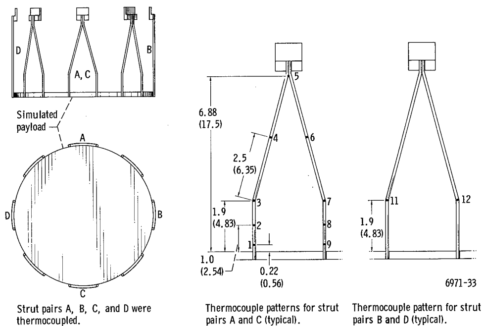
Figure 11. - Location of 40-gage thermocouples for structural support cage of scale model. Thermocouples 1, 2, 8, and 9 were iron-constantan. Thermocouples 3 to 7, 11, and 12 were copper-constantan. (Dimensions are in inches (cm).)
