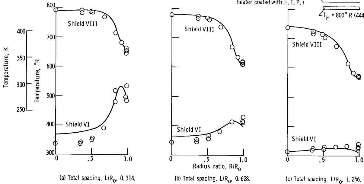
Figure 21. - Effect of targeting and spacing on shield temperature profiles (shields VI and VIII).
