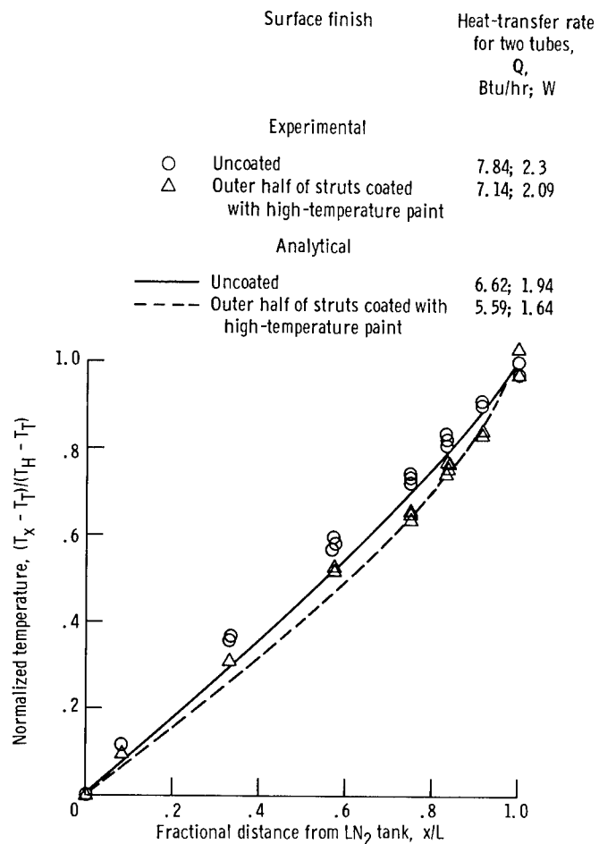
Figure 25. - Effect of external emissivity on temperature of 6-inch-long (15.2-cm-long) stainless-steel tube. Radiant heat transfer from shields <0.1 Btu/hr (0.0293 W).
