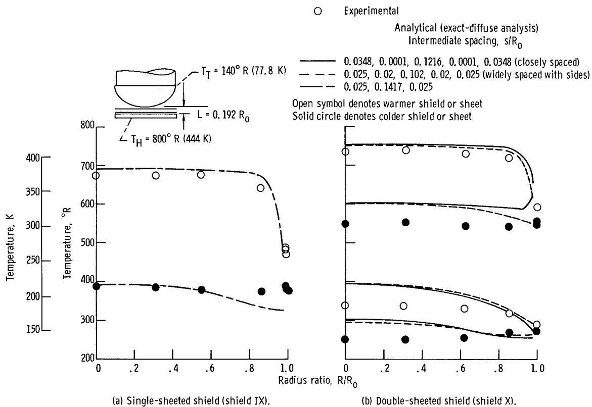
Figure 30. - Temperature profiles of single- and double-sheeted shields for scale-model configuration.
