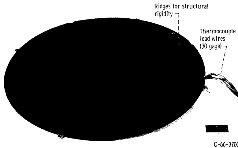
Figure 4. - Construction method for 0.015-inch (0.0381-cm) stainless-steel shield (shield V).
