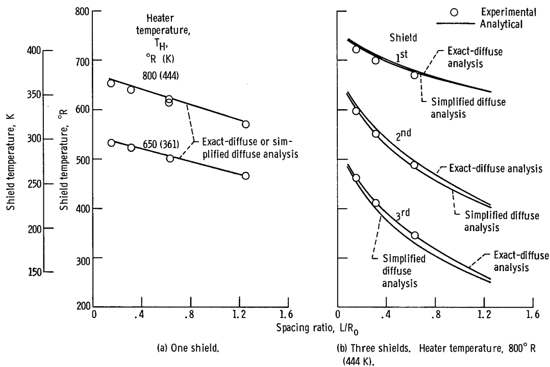
Figure 18. - Effect of spacing ratio on average shield temperatures for one and three intermediate-emissivity shields (shield II).
