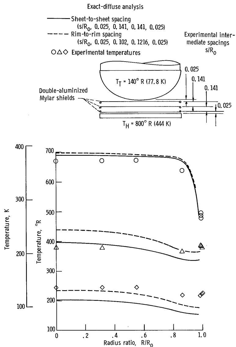
Figure 29. - Temperature profiles for three-shield con- figuration using double-aluminized Mylar shields (shield IX). L/R_0 = 0.332 .
