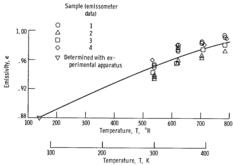
Figure 12. - Emissivity as function of temperature for high-temperature paint. Standard deviation, \pm 0.0089 .
