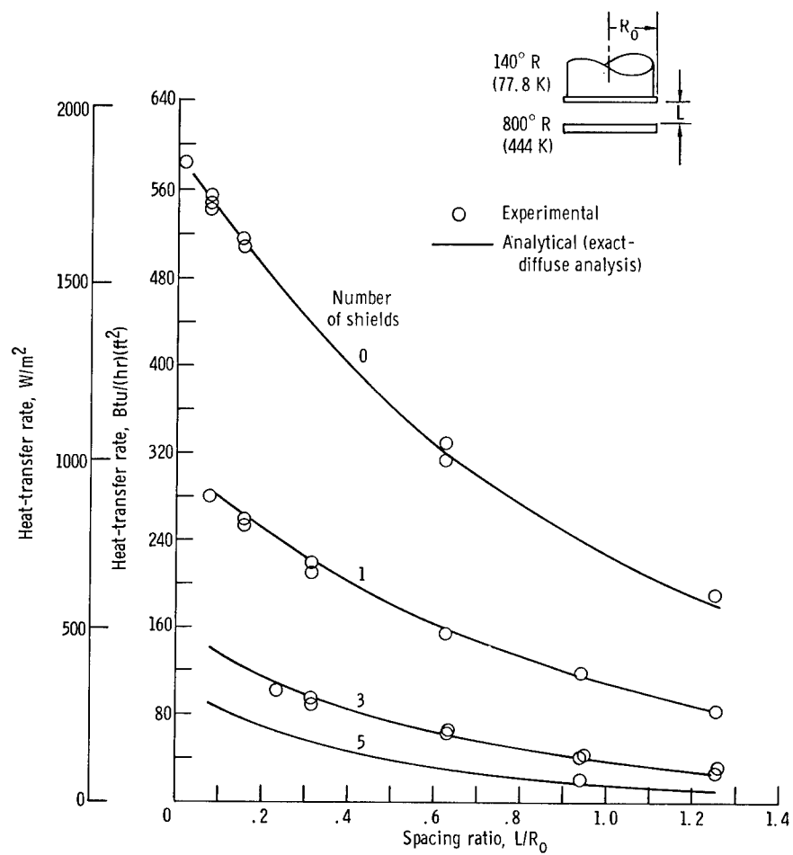
Figure 15. - Effect of shield number and spacing ratio on shadow shield heat-transfer rate. (Shield I.)
