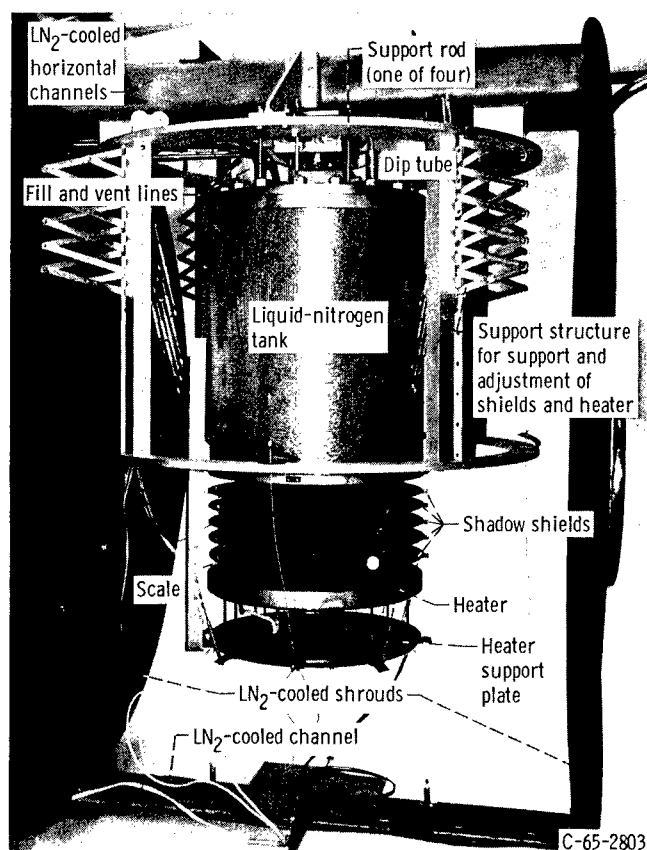
Figure 1. - Apparatus used for a five-shield test.
