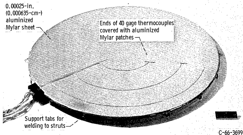
Figure 10. - Double-sheeted shield with structural support welding tabs.
