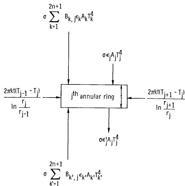
Figure 36. - Sketch showing conductive and radiant heat transferred into annular elemental area of shield. A_j = A'_j ; T_j = T'_j .
