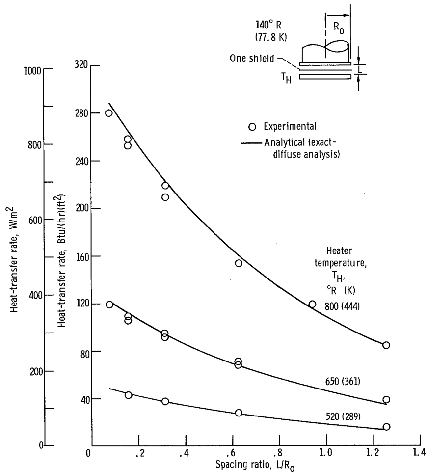
Figure 14. - Heat-transfer rate as function of spacing ratio and heat-source temperature for one shadow shield (shield I).
