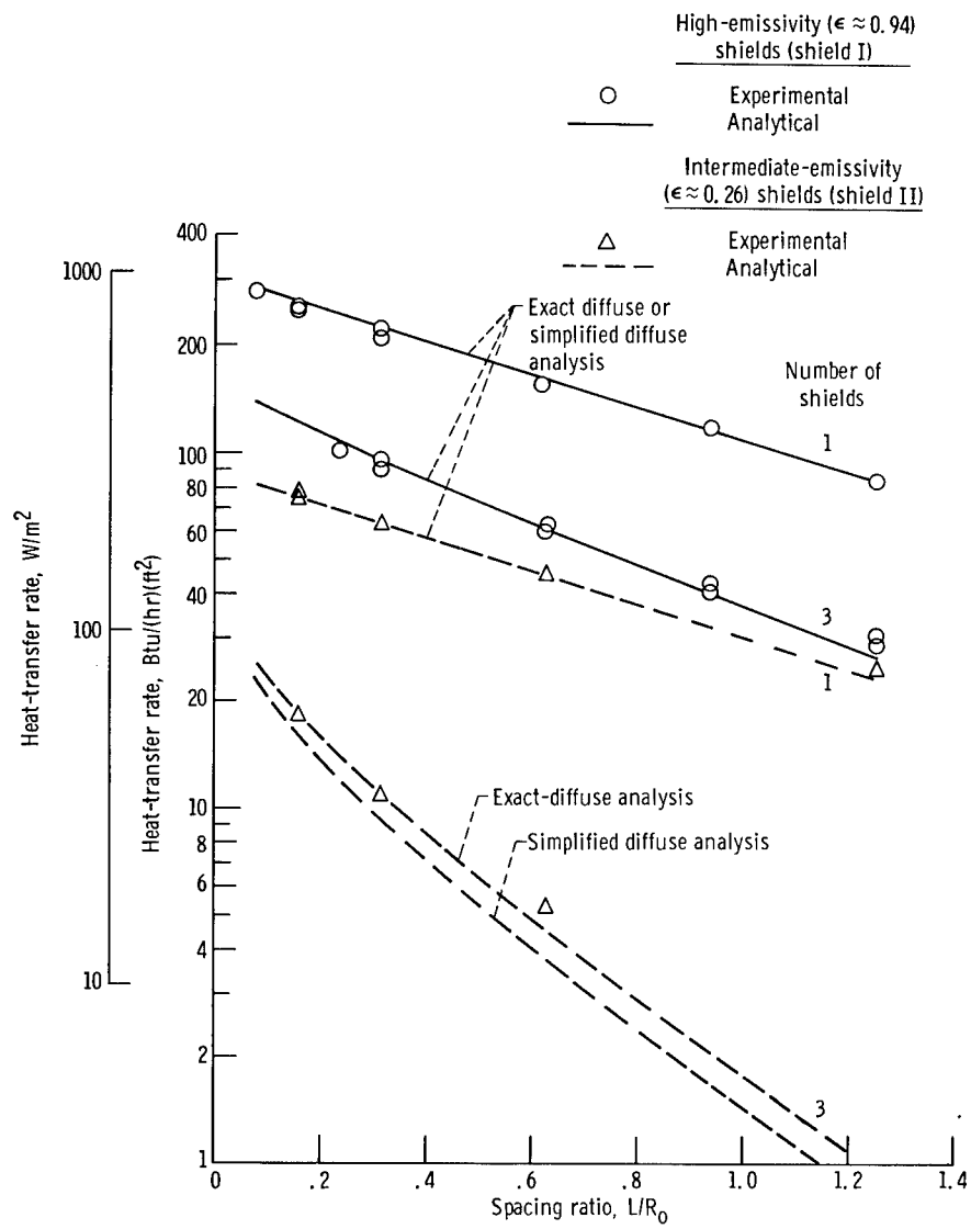
Figure 17. - Effect of shield emissivity and spacing ratio on heat-transfer rate for high-conducting shields (shields I and II). (Heater temperature, 800^\circ R ( 444 K )).
