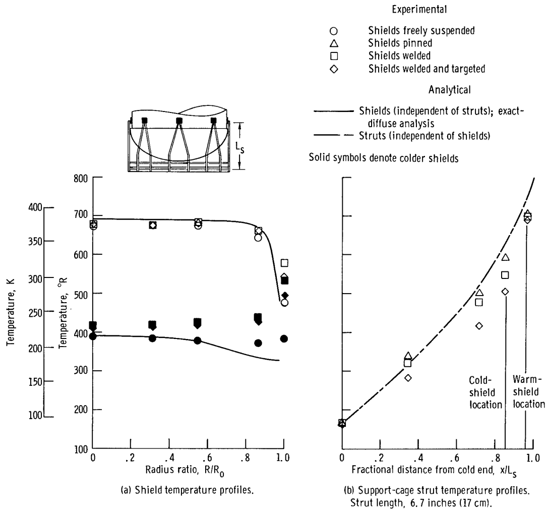
Figure 32. - Shield and support-cage temperature profiles for pinned, welded, and targeted systems (shield IX). L/R_0 = 0.192 .
