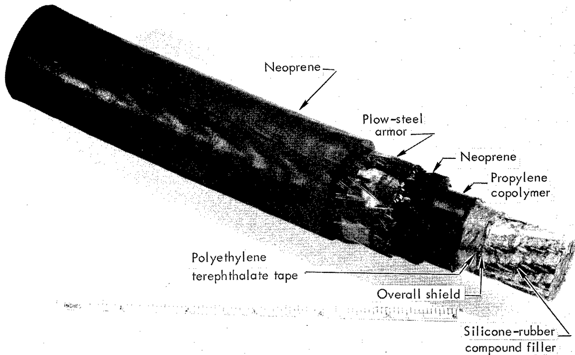
Fig. 2. Cutaway view of Gasbuggy arming and firing cable.
