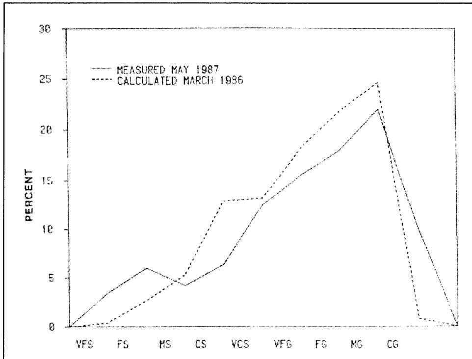
Figure 11. Bed-material gradation between stilling basin and College of Marin Bridge
