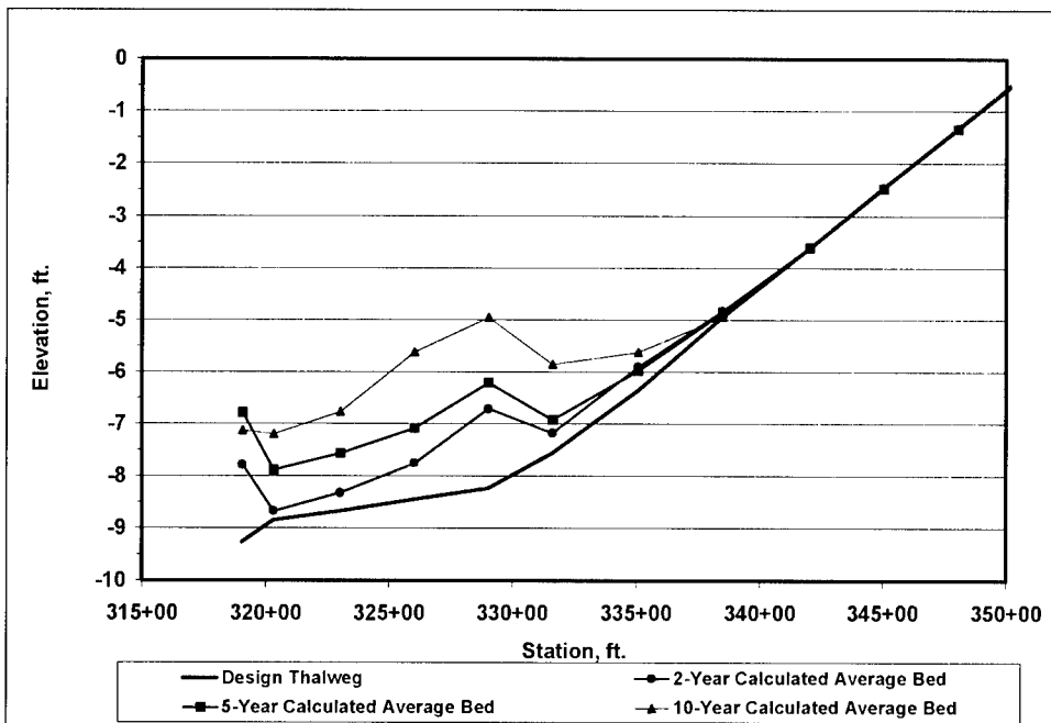
Figure 21. Antecedent aggradation in concrete channel – Type 19 Design
