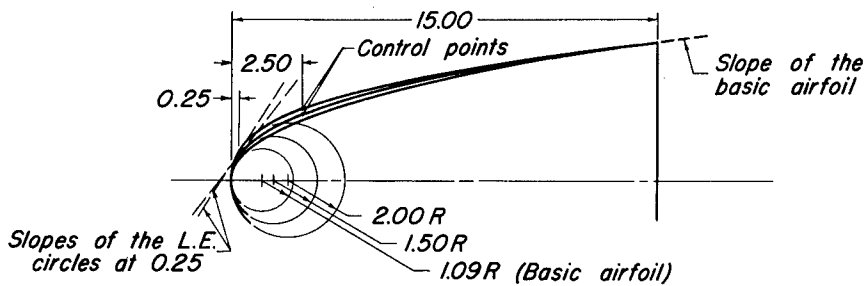
(b) Design details for modifications 1 & 2.
