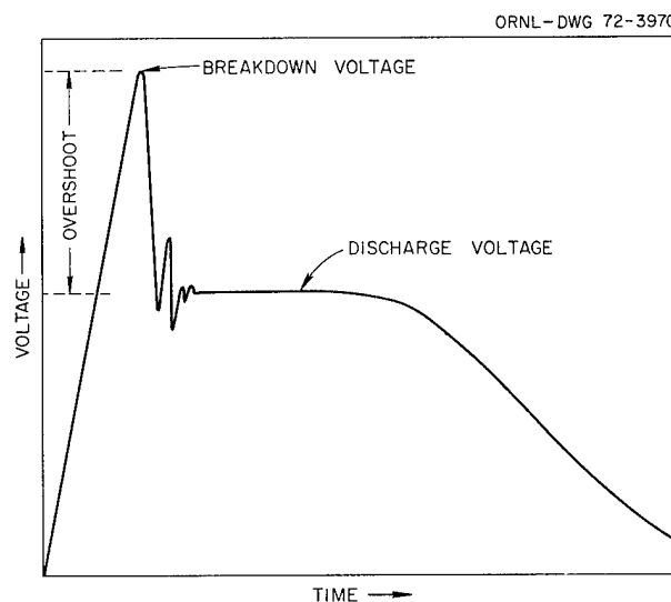
Fig. 17.15. Time history of voltage across a lightning arrester illustrating the distinction between breakdown voltage and discharge voltage in the situation where the magnitude of the former exceeds that of the latter.
