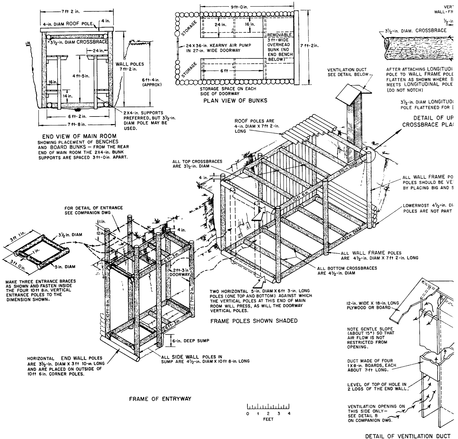
Pictorial View of Small-Pole Shelter. Fig. 13.1. Pictorial view of hasty pole shelter.
