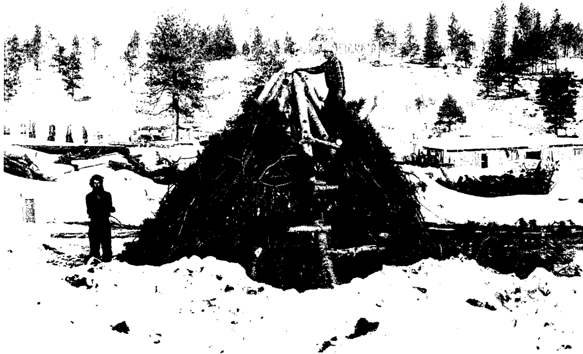
Fig. 14.1. Log-Tepee Shelter built according to modified Russian specifications and dimensions given in an article by F. Ostroukh: "Winter Shelters," in Voyennyye Znaniya , No. 2, February 1971, Moscow. Twelve logs, each 17 ft long and with 6- to 10-in.-diam tops, were tied together around their tops with approximately 200 ft of \frac{1}{4} -in. nylon cord. Later, the covering of pine limbs (over the wired-on short horizontal poles) was completed, except for the entryway opening, in which a man is seen squatting.
