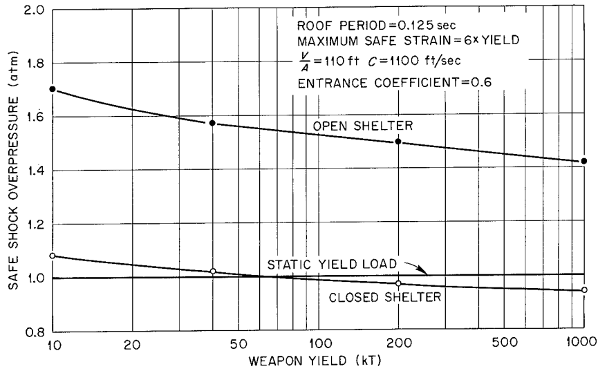
Fig. 13.14. Weapon yield vs shock overpressure.
