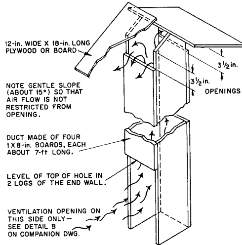
DETAIL OF VENTILATION DUCT
