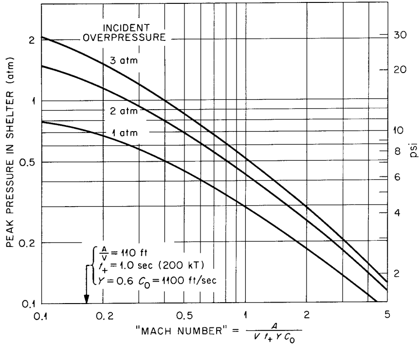
Fig. 13.15. Peak pressure in shelter vs Mach No.
