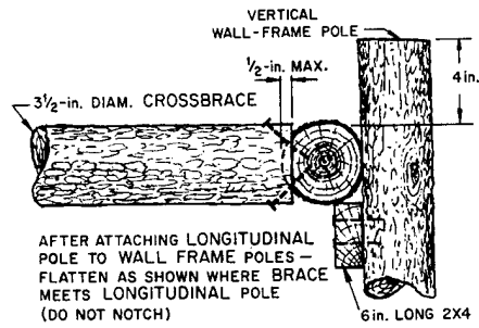
3 1/2-in. DIAM LONGITUDINAL POLE FLATTENED FOR BRACE DETAIL OF UPPER CROSSBRACE PLACEMENT
