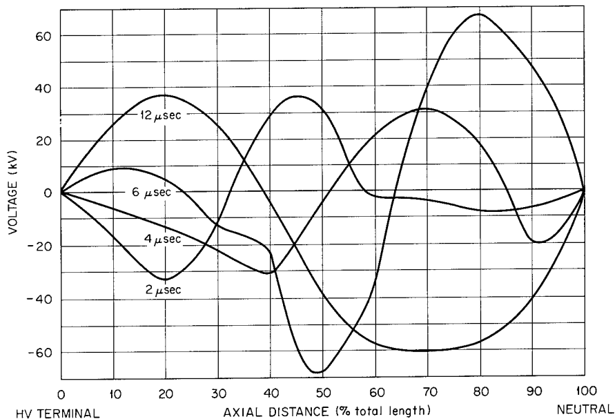
Fig. 17.18. Voltage in the secondary winding vs axial distance into the winding for times of the order of the first natural period of the winding.
