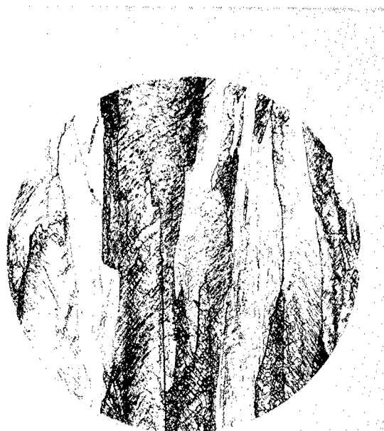
(a) As-swaged; before rupture. X75. (b) Recrystallized in hydrogen; before rupture. X75.
