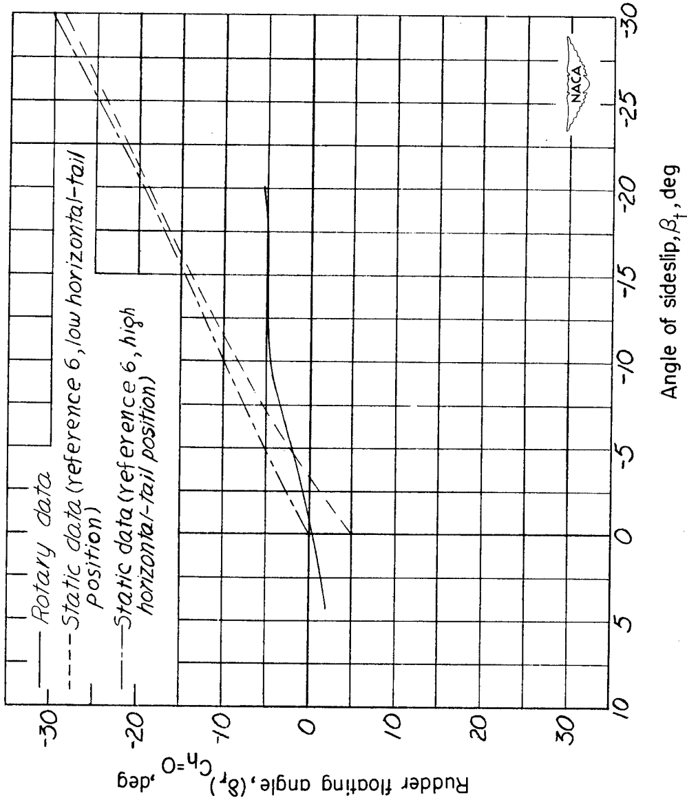
(a) \alpha = 15^\circ .
