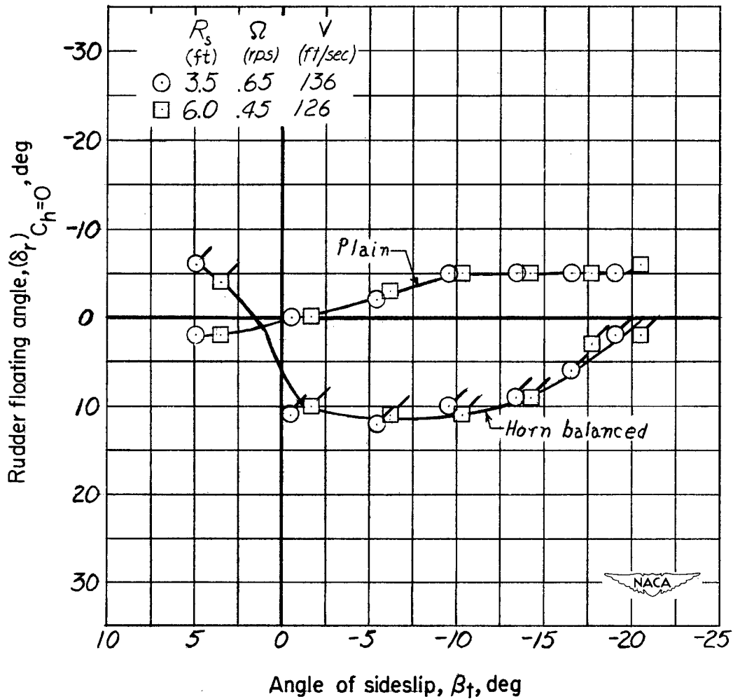
(a) \alpha = 15^\circ .
