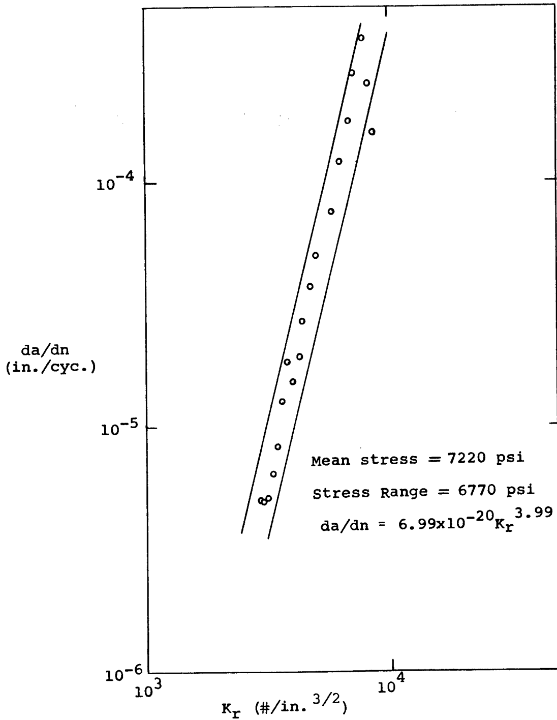
FIGURE 12 da/dn vs. K_r Shell #10
