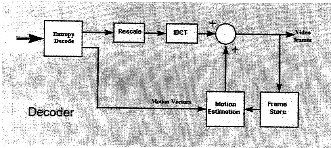
Figure 2.3 H.263 Decoder
