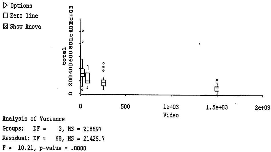
Figure 5.10 Bandwidth Affect on Error
