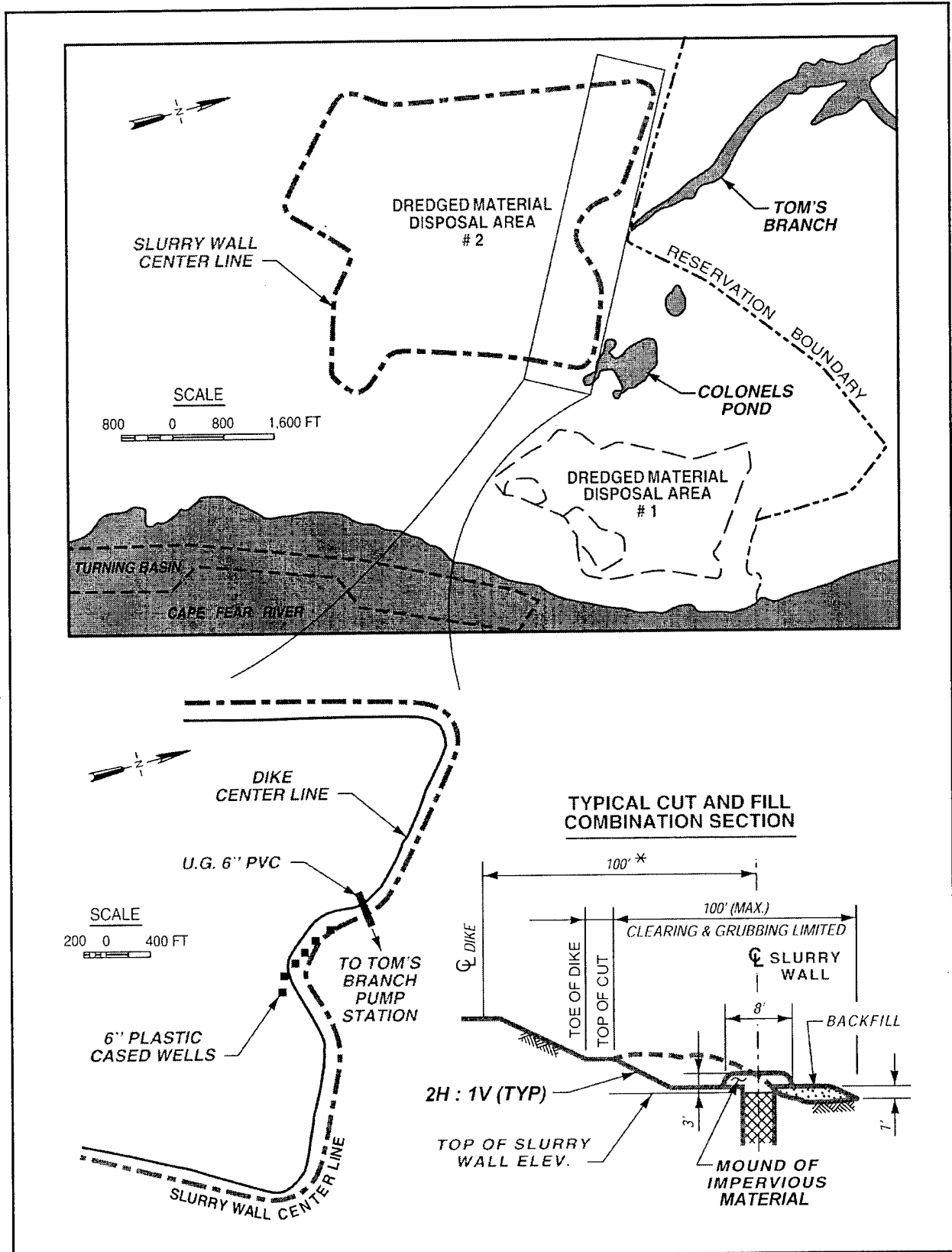
Figure 25. Plan and cross-sections of Sunny Point CDF showing slurry wall configuration
