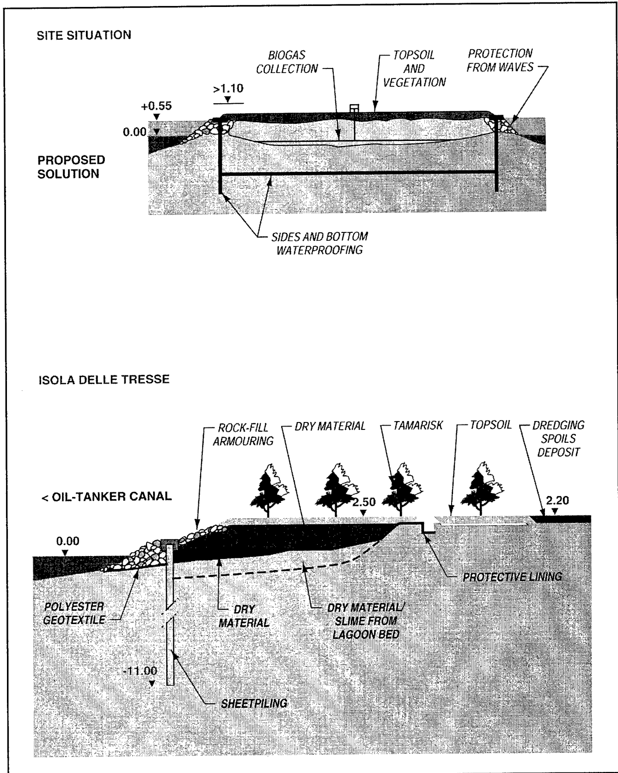
Figure 17. Tresse Island CDF, Venice, Italy, showing typical perimeter dike cross-section
