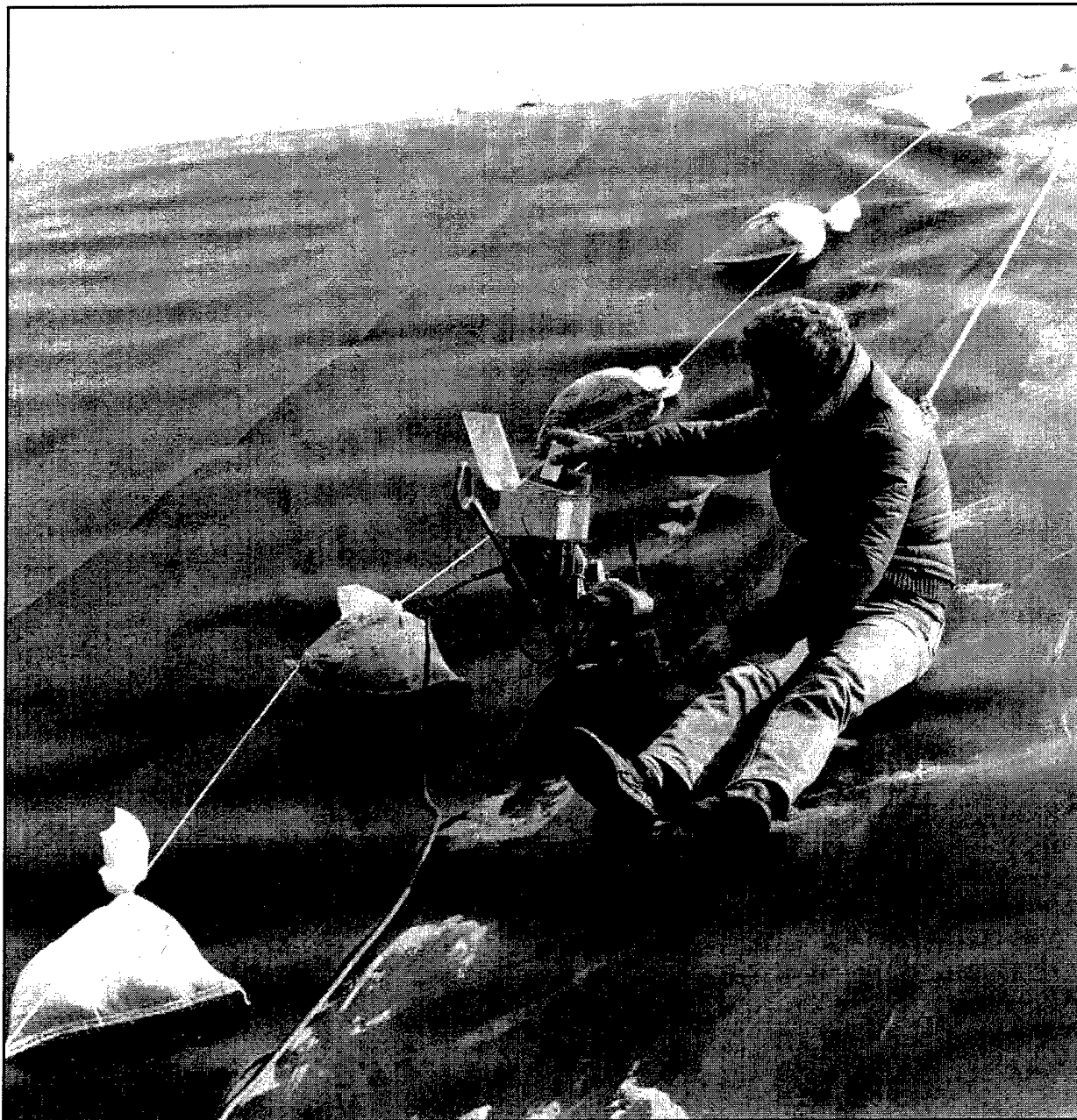
Figure 16. Heat welding liner, Parrot's Beak CDF, Rotterdam
