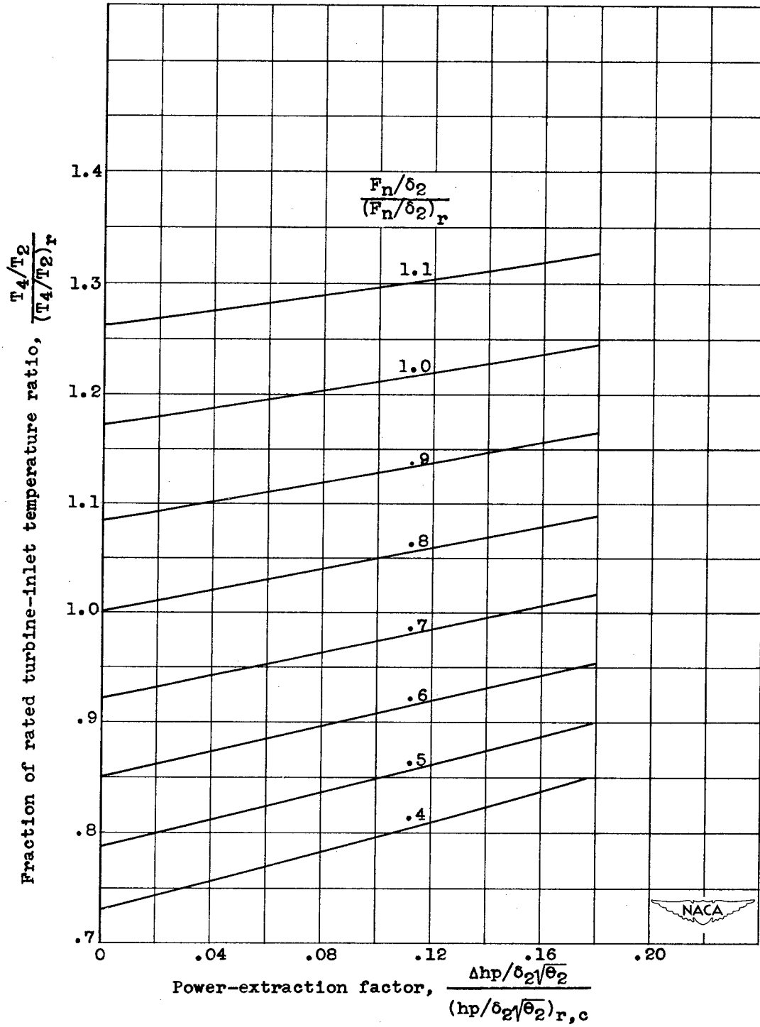
Figure 1. - Continued. Variation of turbine-inlet temperature ratio with power extraction and thrust for variable-area tail-pipe nozzle and ram pressure ratio of 1.35.
