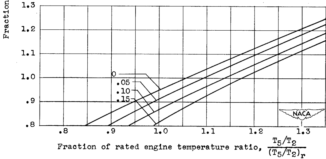
(b) Corrected engine speed, rated.
