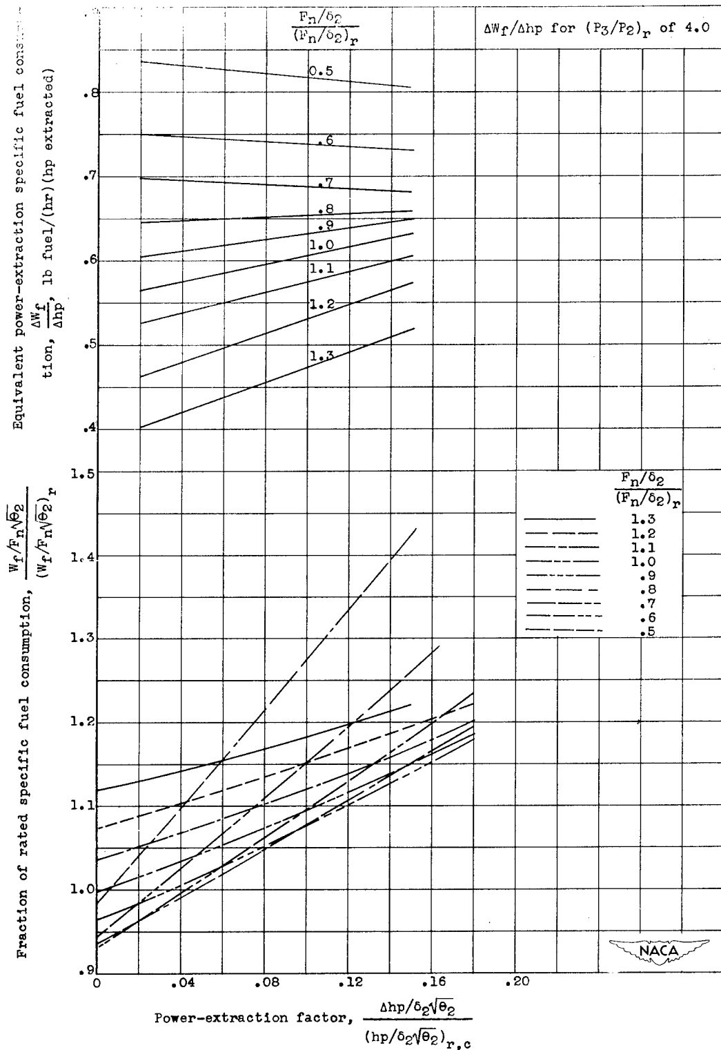
(b) Corrected engine speed, rated.
