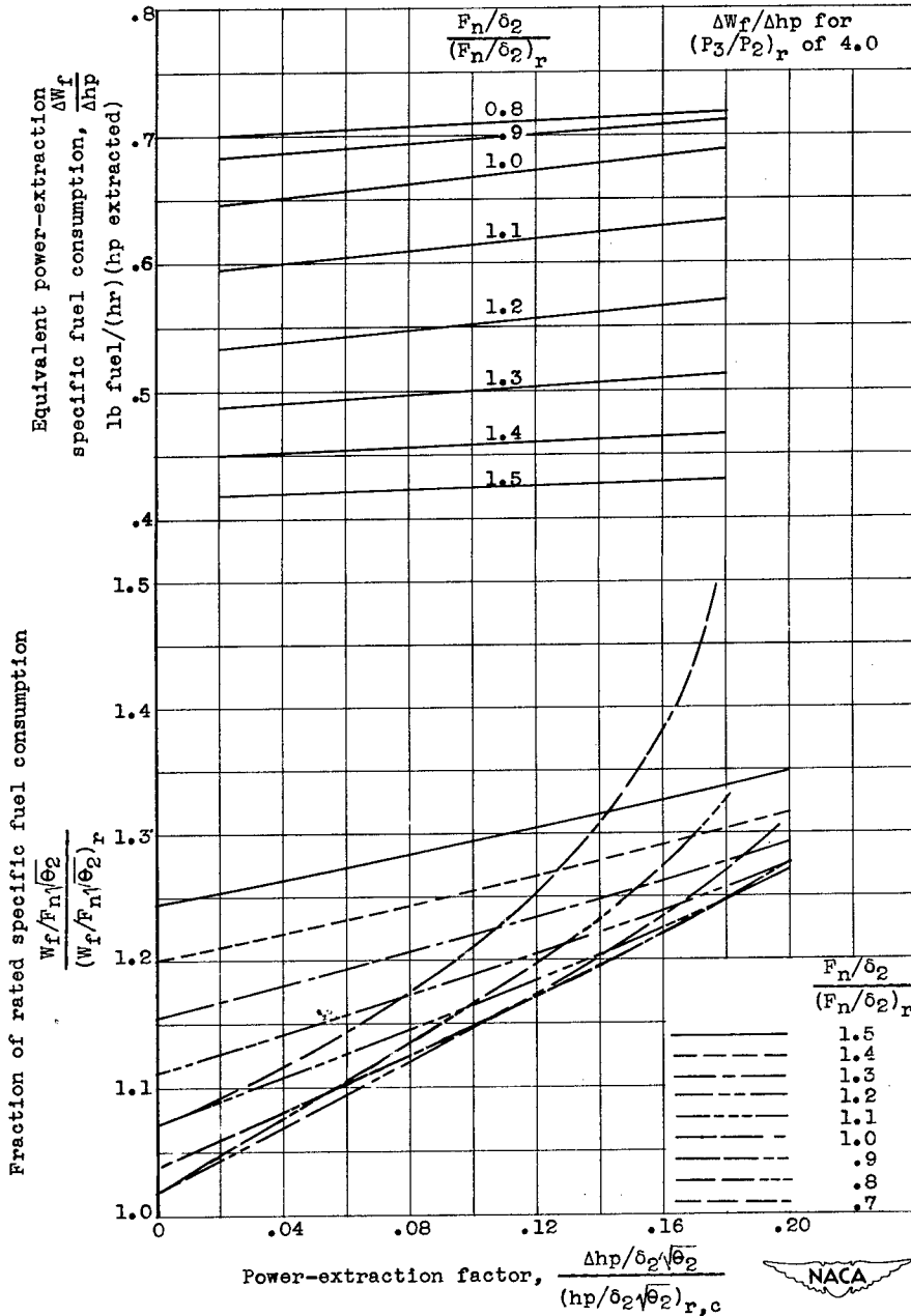
(c) Corrected engine speed, 1.1 rated.
