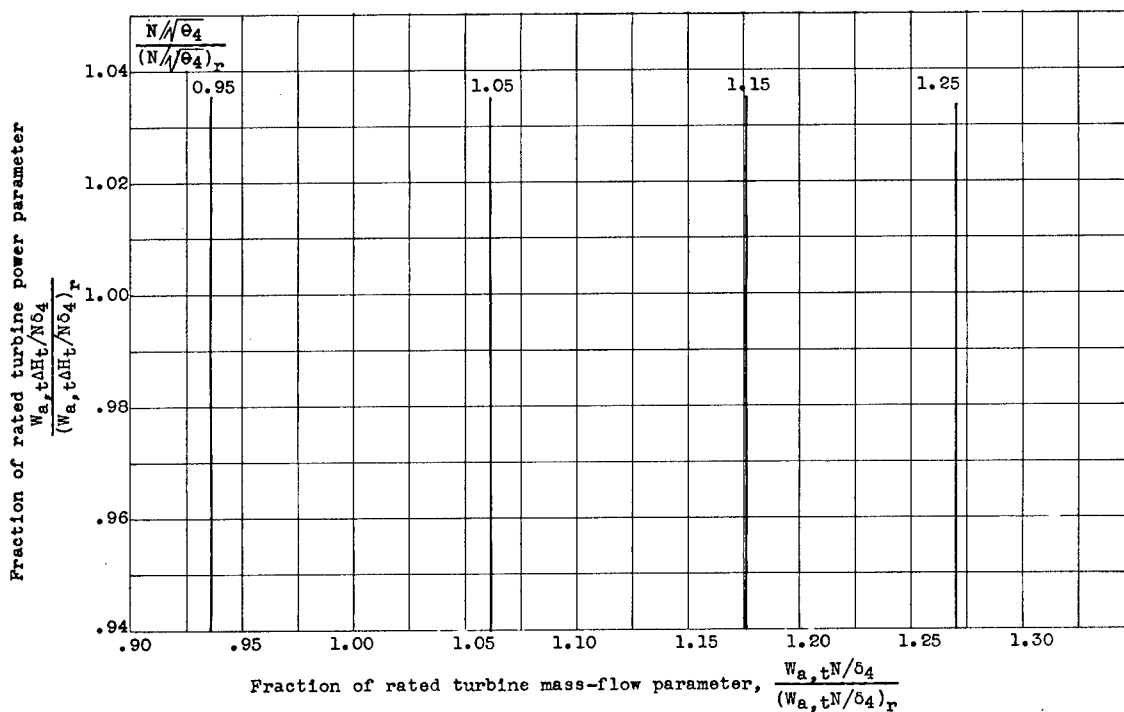
Figure 14. - Idealized turbine characteristics.
