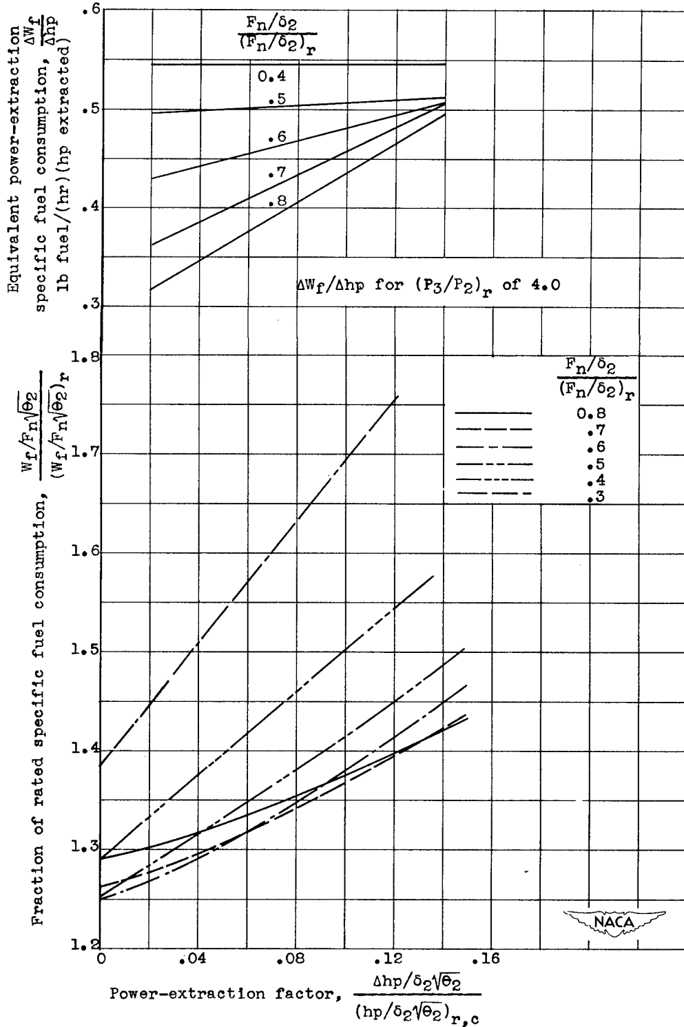
(a) Corrected engine speed, 0.9 rated.
