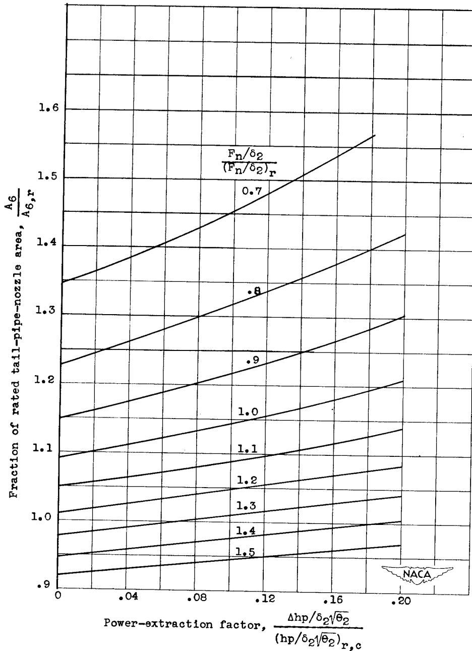
Figure 5. - Concluded. Variation of tail-pipe-nozzle area with power extraction and thrust for ram pressure ratio of 0.99.
