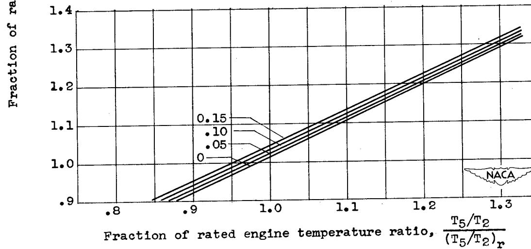
(c) Corrected engine speed, 1.1 rated.
