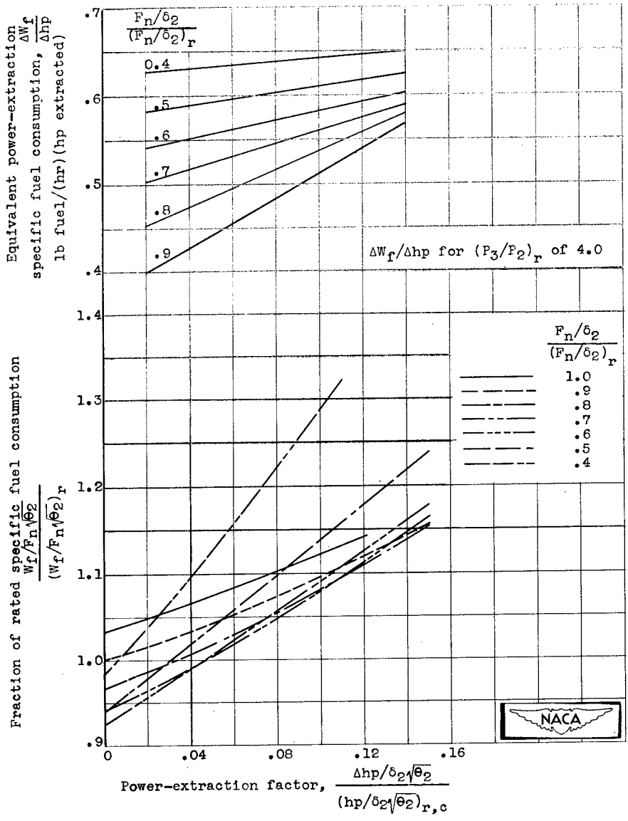
(a) Corrected engine speed, 0.9 rated.
