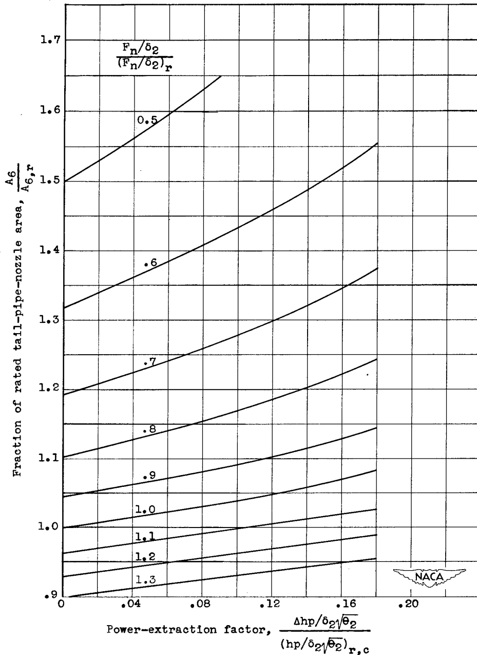
(b) Corrected engine speed, rated.
