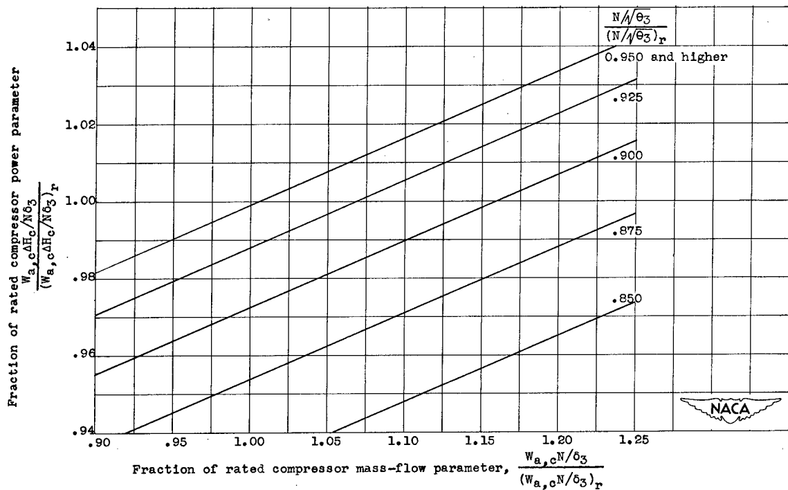
Figure 13. - Idealized axial-flow compressor characteristics.
