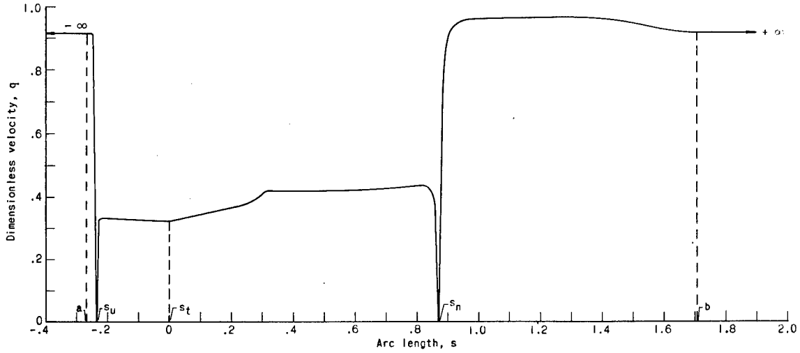
Figure 9. - Velocity distribution for second slotted blade.
