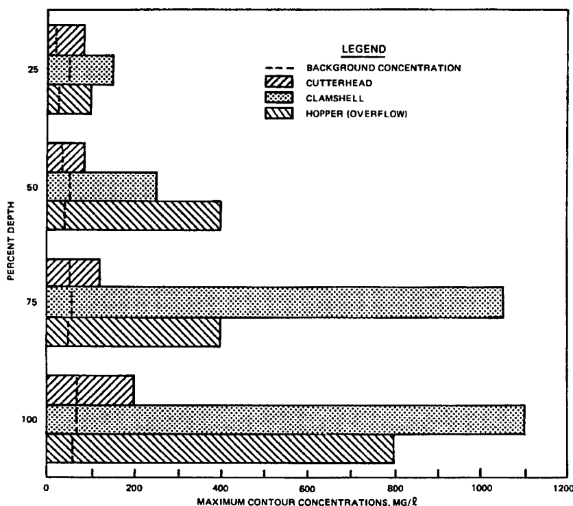
Figure 5. Maximum TSS concentration levels (milligrams/litre) measured for cutterhead, clamshell, and hopper dredges during IOMT field studies
