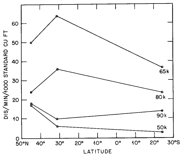
Fig. 7b—Variation of Sr 90 activity with latitude.
