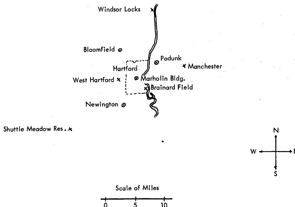
Fig. 14—Pot fallout collections in the Hartford area. \odot , pot fallout collecting stations; x, rain measurement stations.
