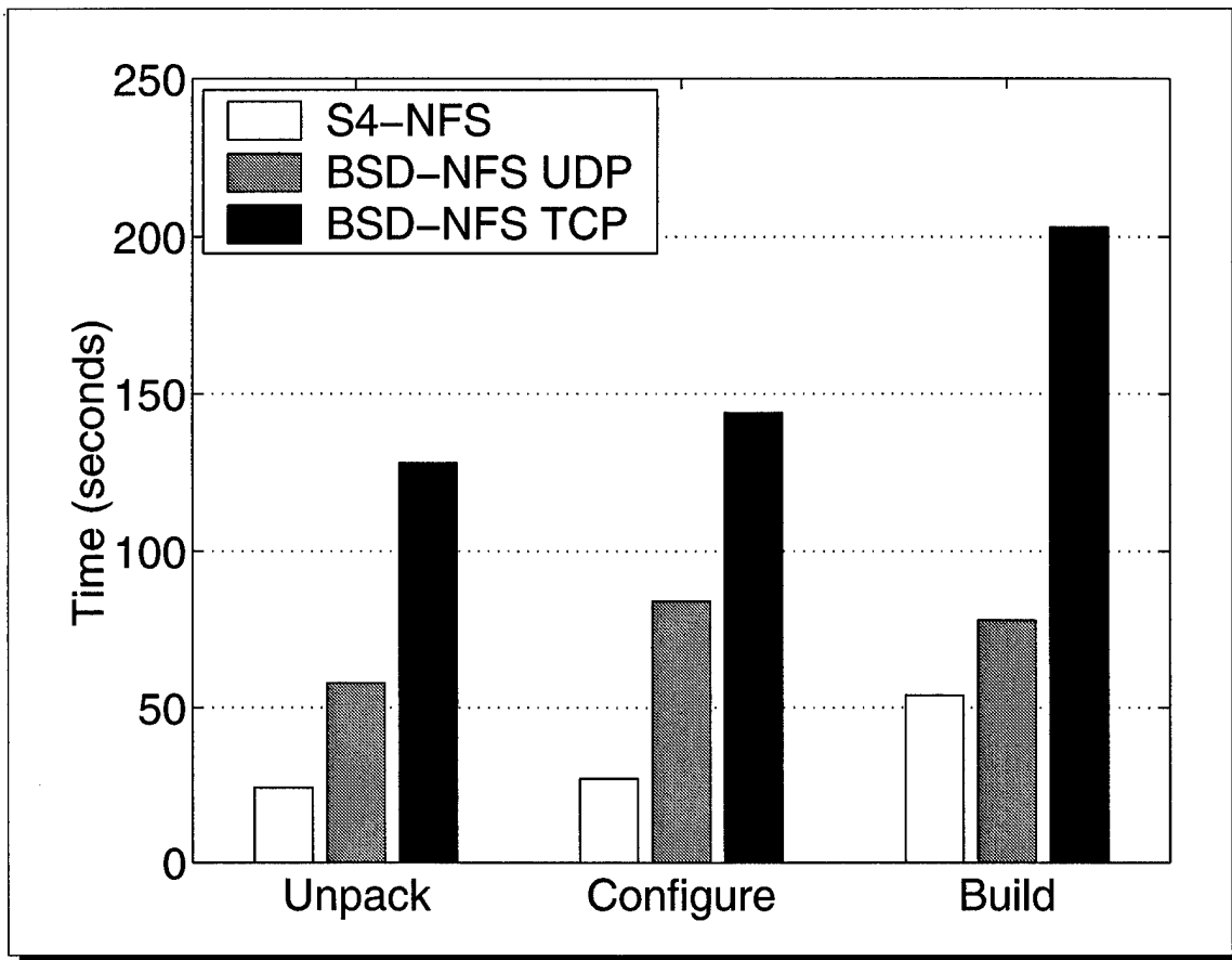
Figure 10: SSH - Unpack, configure, and build.
