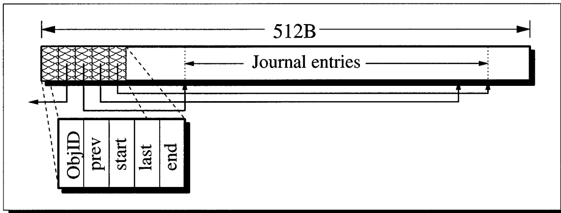
Figure 4: Journal sector. Contains packed journal entries.
