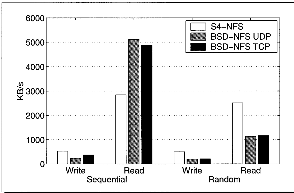
Figure 8: Large-file performance.
