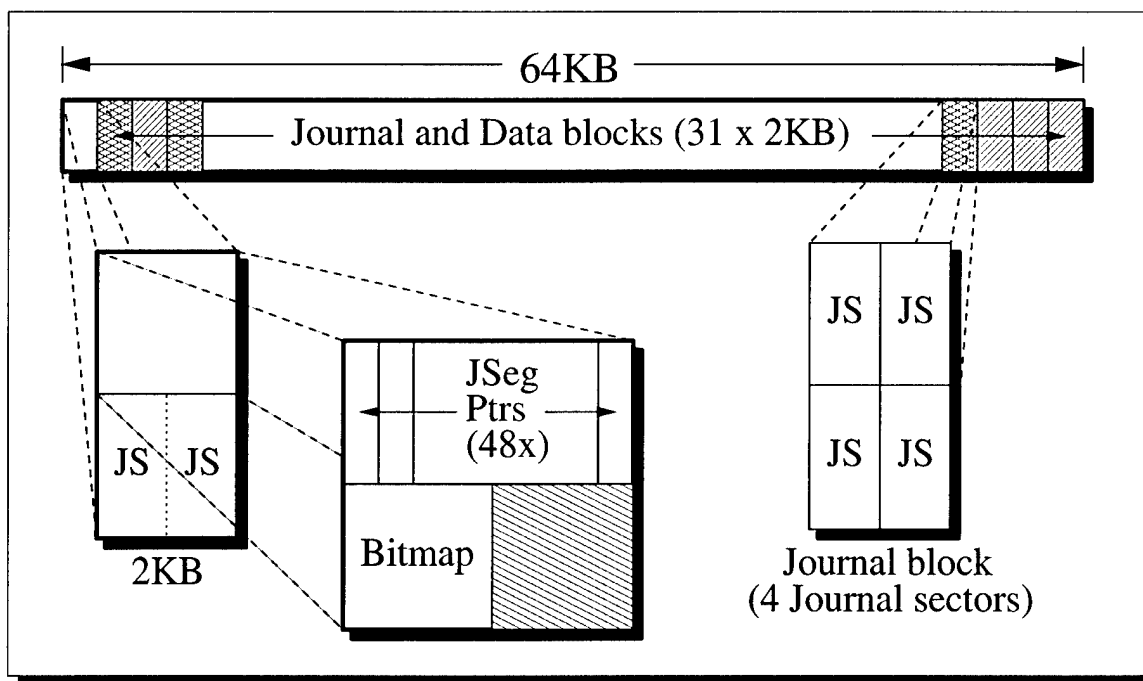
Figure 3: Data Segment . This structure holds all log data.
