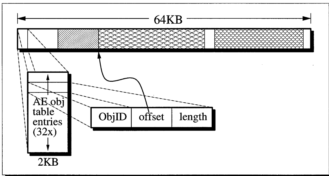
Figure 5: Anti-entropy segment. Holds the anti-entropy caches for various objects.
