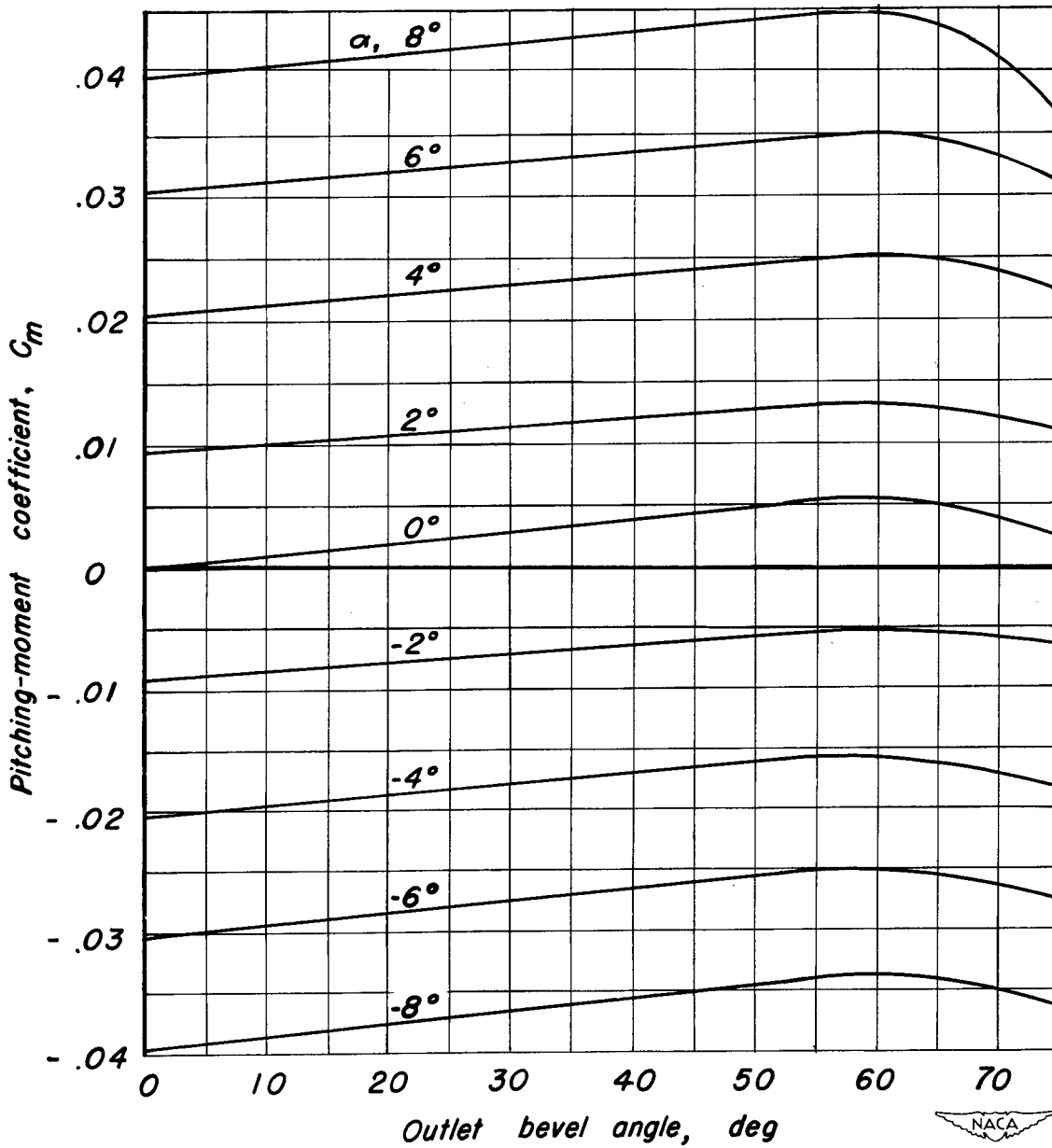
Figure 8.—Variation of pitching-moment coefficient with outlet bevel angle from jet-off tests. V_j/V_0, 0 .
