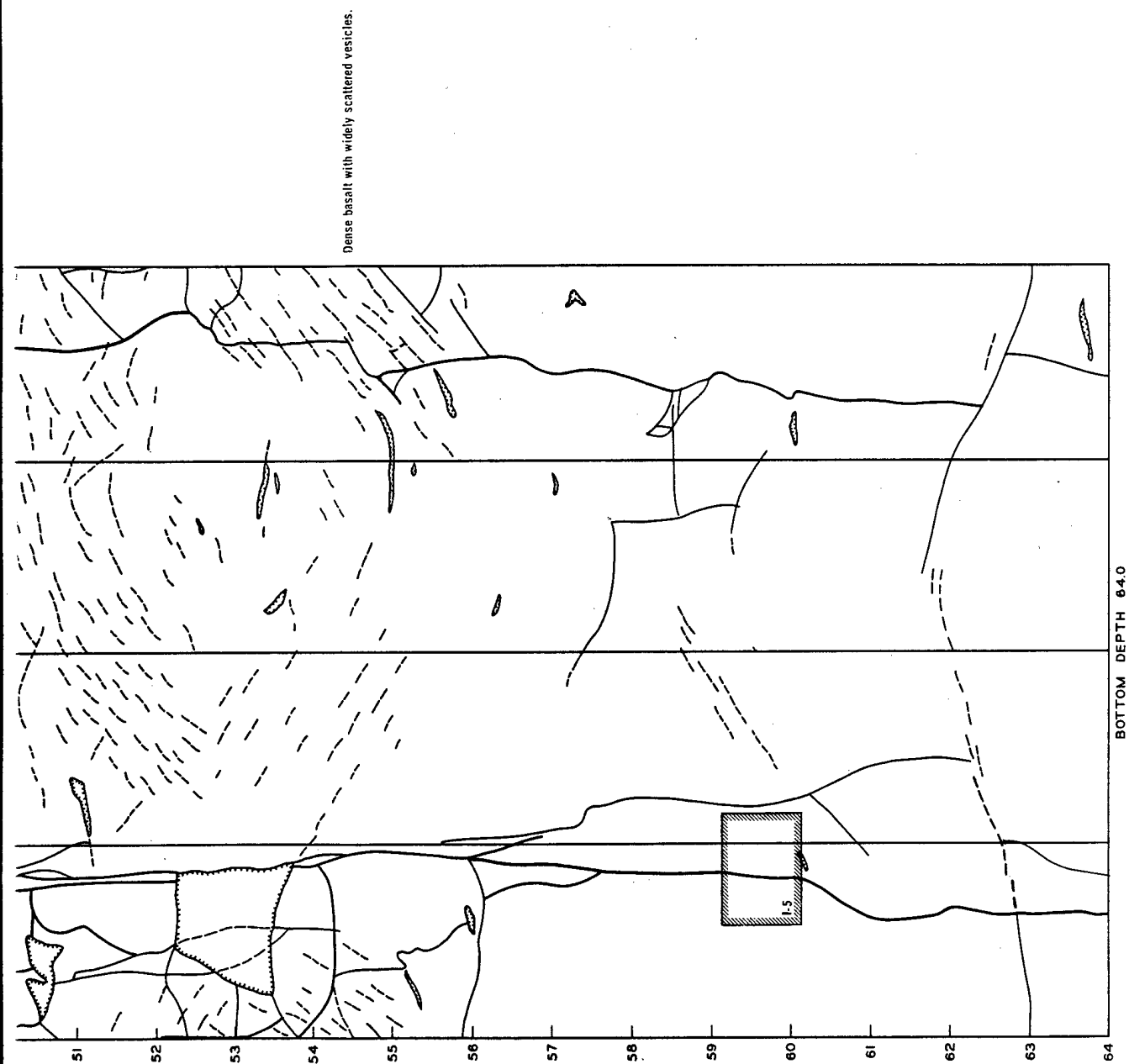
Figure B.6 Log of calyx Hole U181 (Continued).
