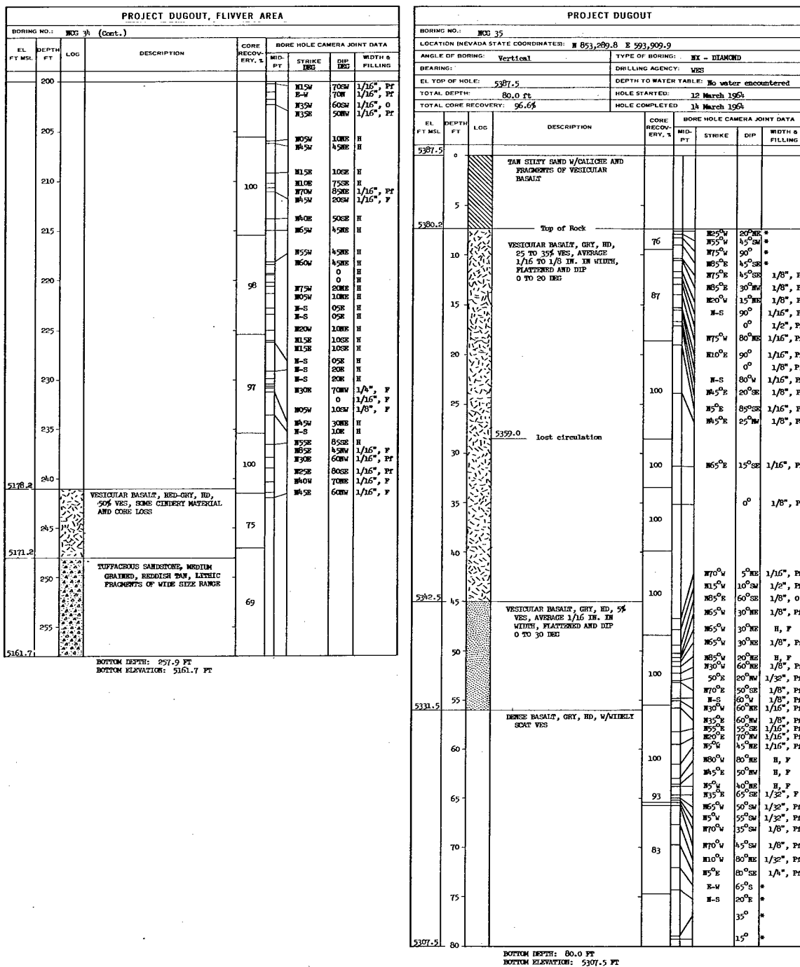
Figure A.17 Logs of core Borings NCG 34 (Continued) and NCG 35.
