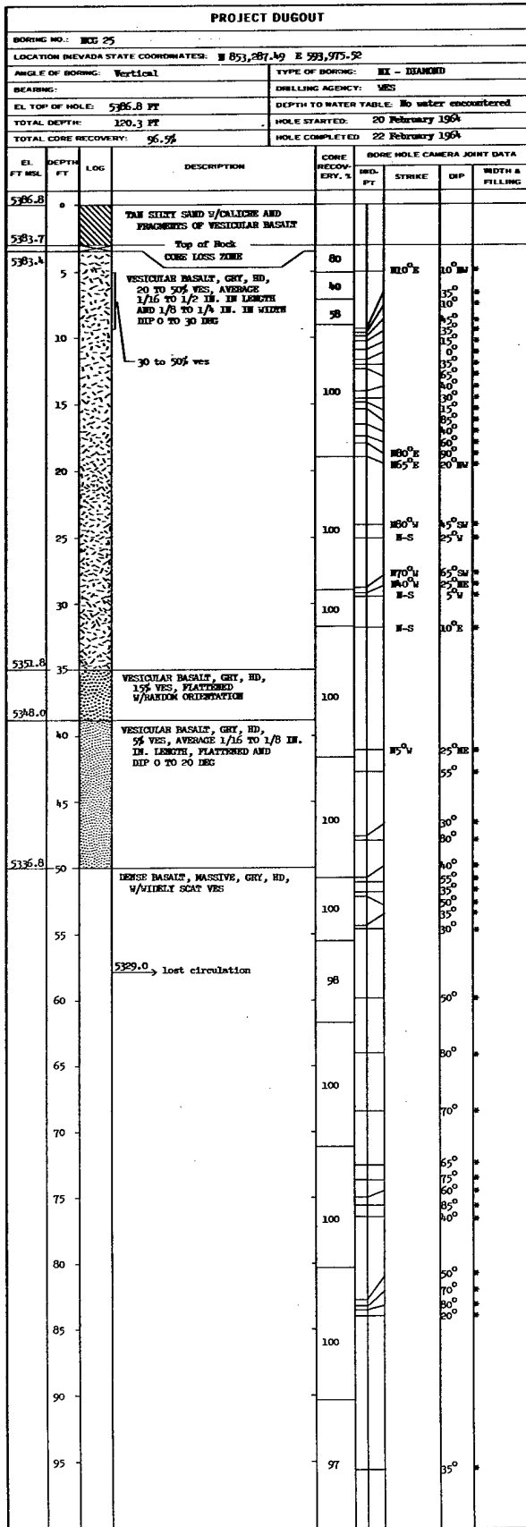
Figure A.9 Log of core Boring NOG 25.
