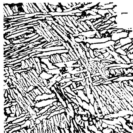
FIGURE 23 - ELECTRON BEAM WELDED NOTCHED TENSILE SPECIMEN ( BETA FORGED ) AFTER TESTING, SHOWING PROFILE OF FRACTURE ( UPPER PHOTO ) AND MICROSTRUCTURES ( LOWER PHOTOS ) OF THE THREE ZONES NOTED, ( 1 ) BASIS METAL, ( 2 ) HEAT AFFECTED ZONE, AND ( 3 ) WELD METAL.
