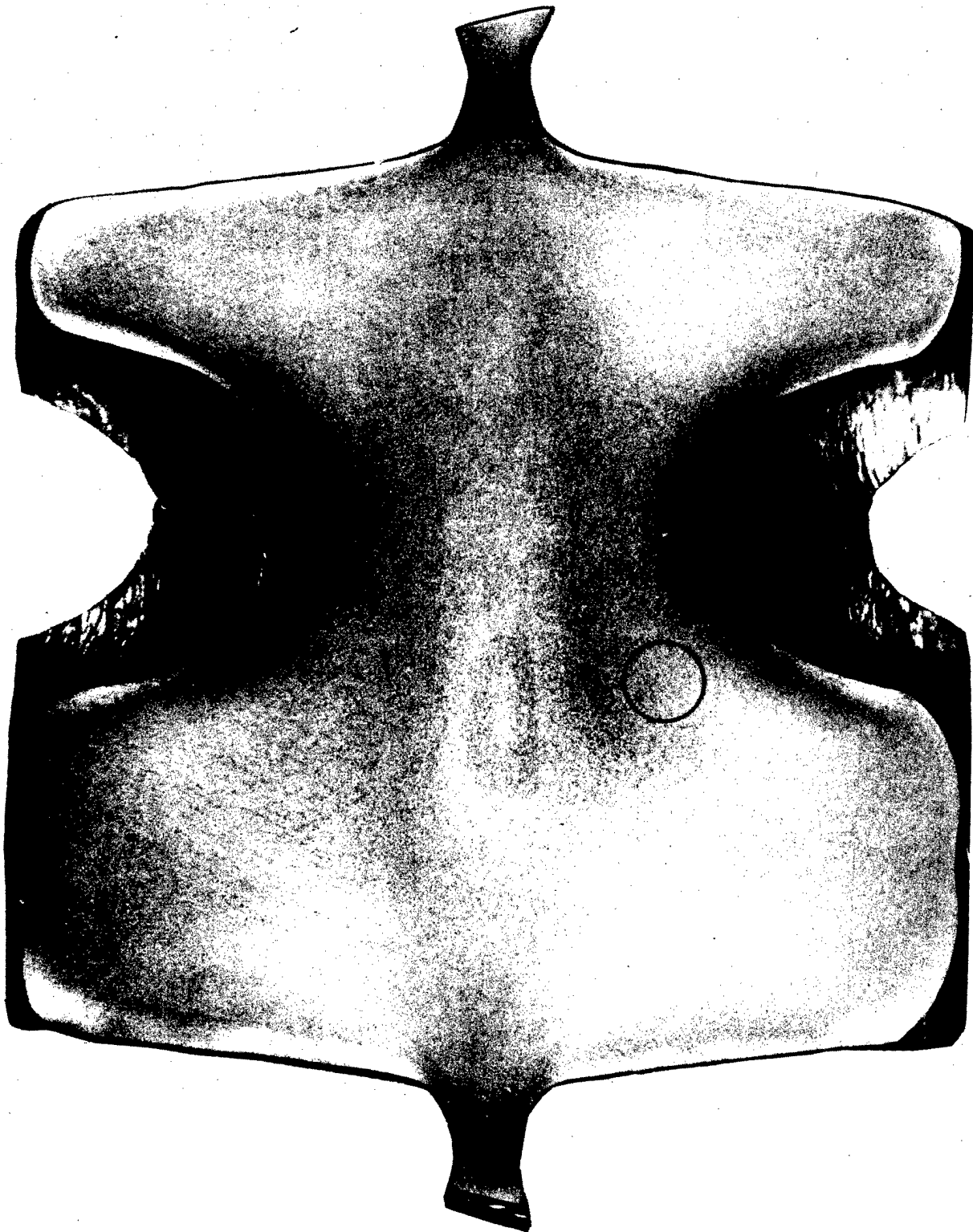
FIGURE 19 - SECTION CUT THROUGH HEAVY CENTER PORTION OF ALPHA-BETA FORGING TO SHOW GRAIN FLOW PATTERN. CIRCLED AREA IS LOCATION OF MICROSTRUCTURE SHOWN IN FIGURE 20.
