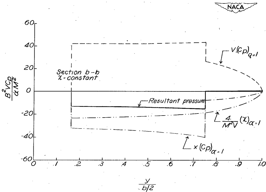
(c) Sonic leading edge, supersonic trailing edge.
