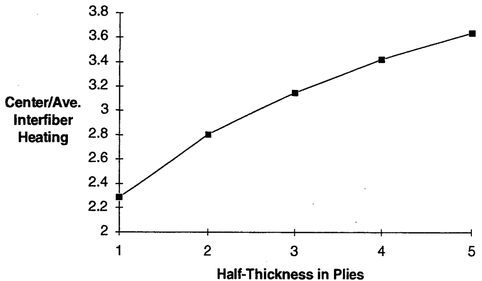
Figure 10. Ratio of Center to Average Interfiber "Heating," \gamma_1 / [(\gamma_{total} - \gamma_1) / (m + n)] , Plotted Against Increasing Ply Thickness. This Represents the Multiplicity of Average Interfiber Heating That Is Consumed by the Interply Resin. For Example, at a Laminate Thickness of 2 Plies (Half-Thickness = 1), the Heating in the Interply Resin-Rich Region Is Approximately 2.3 Times the Average Heating in the Rest of the Laminate.
