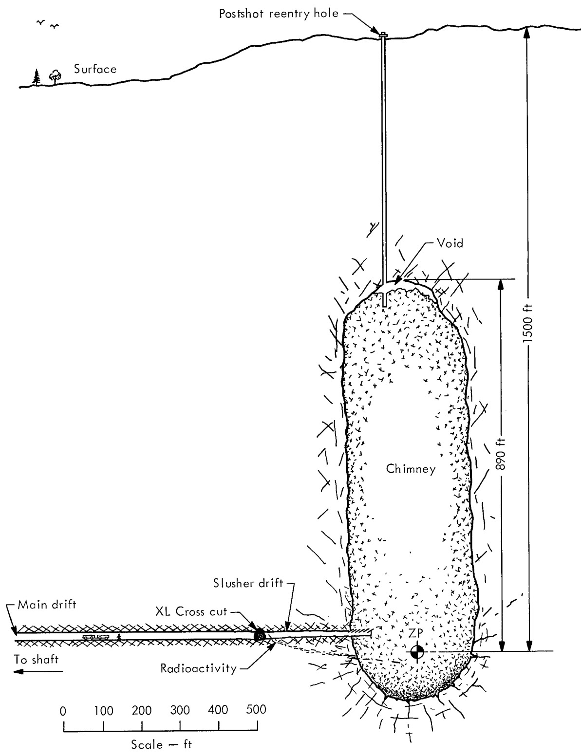
Fig. 1. Elevation view of post-Piledriver.
