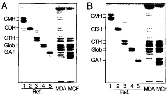
Figure 1. Neutral glycolipids of MDA-MB-231 and MCF-7 human breast cancer cells. Neutral glycolipids were separated by TLC with chloroform/methanol/0.2% CaCl 2 (60:35:8) in A and chloroform/methanol/2.5 N NH 4 OH (60:35:8) in B, and visualized with 20% sulfuric acid. MDA, neutral glycolipids of MDA-MB-231 cells; MCF, neutral glycolipids of MCF-7 cells. Ref. (reference glycolipids): 1, CMH; 2, CDH; 3, CTH; 4, globoside; 5, asialo-GM1. * Nonglycolipid component which gives a yellowish band with anthrone-sulfuric acid reagent.
