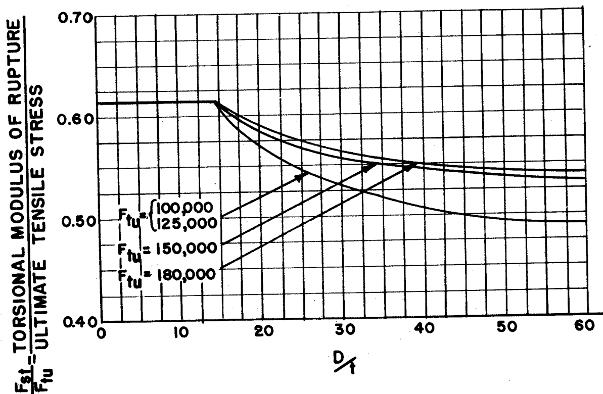
Figure 2.42 (b). Torsional modulus of rupture of round alloy steel tubing.
