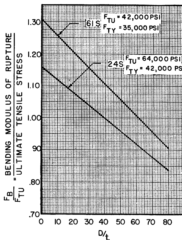
Figure 3.321. Bending modulus of rupture aluminum alloy round tubing restrained against local buckling at loading points.
