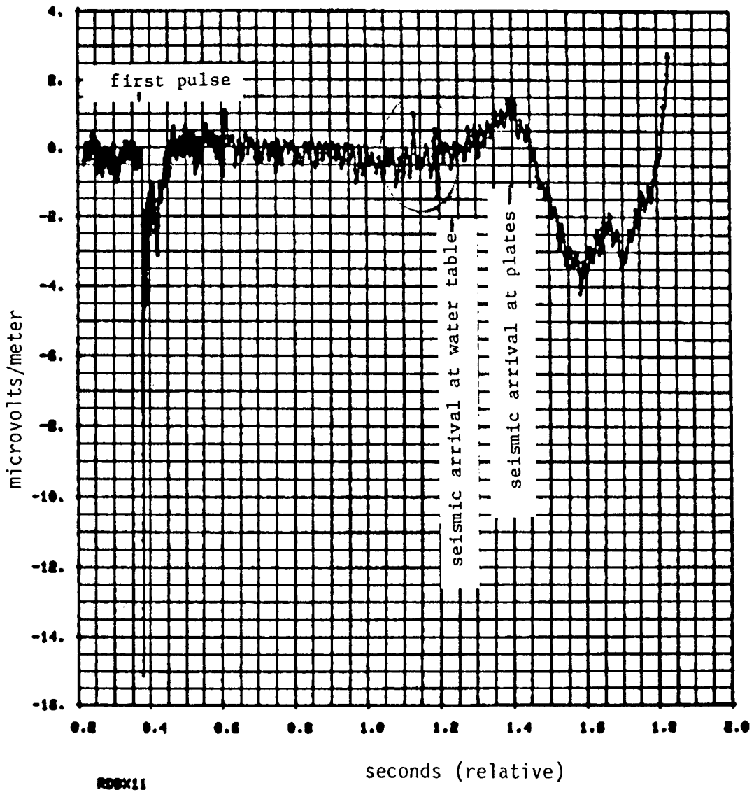
DDX11 Fig. F-5. Draughts Event EMP--Buried plates across Yucca fault. Distance: 4.1 km Azimuth from GZ: N33°W Plate Separation: 150 m Plate Orientation: E-W
