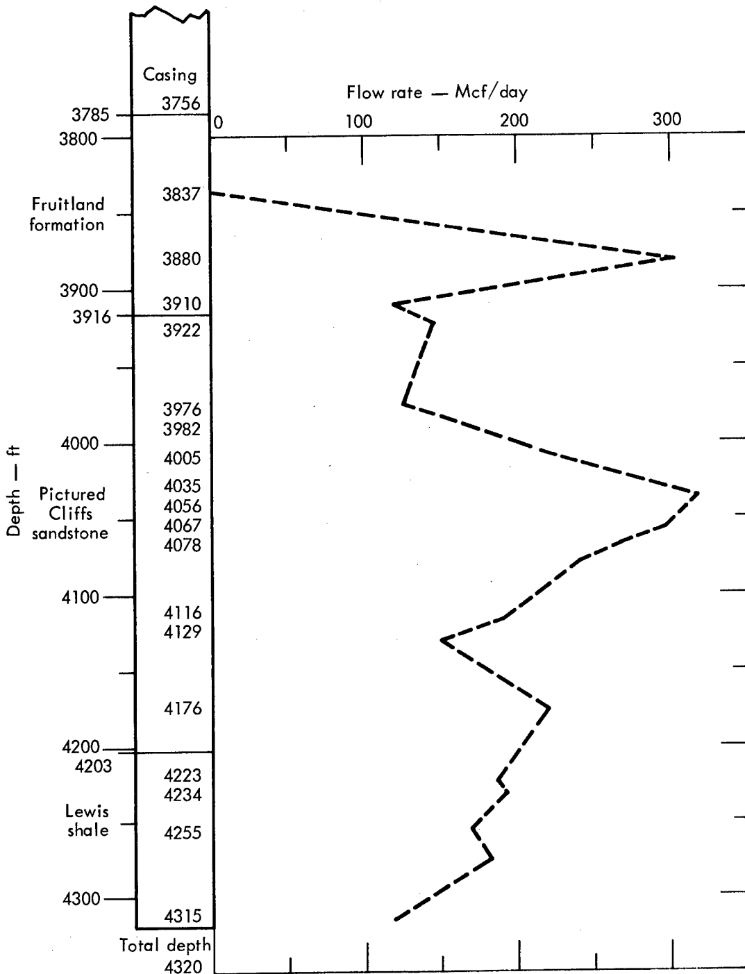
Fig. 7. Natural gas flow rates while core drilling, GB-1.
