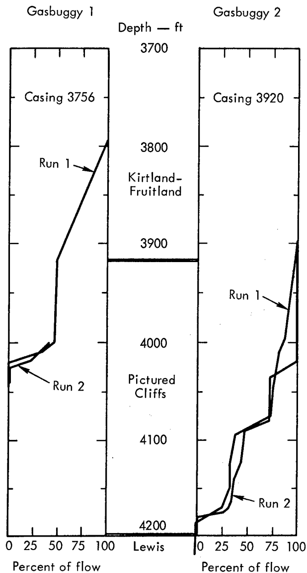
Fig. 8. Integral packer flowmeter logs.
