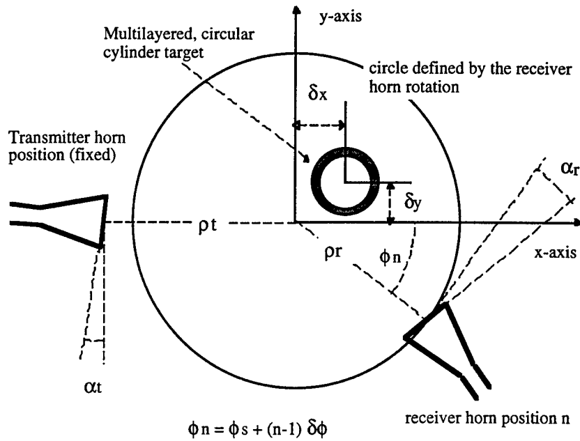
Fig. 3.4.3.3. Illustration of the calibration parameters determined by the calibration algorithm for a single view of a cylindrically symmetric target.
