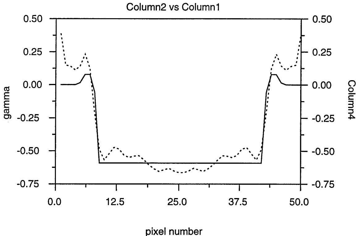
Figure 3.3.3 Comparison of the reconstruction (dashed) with the true dielectric distribution (solid) on an axis through the center of the pipe. Plotted is the scattering potential relative to the sand: \gamma(x, y) = \epsilon_r(x, y) / \epsilon_r(\text{sand}) - 1 .
