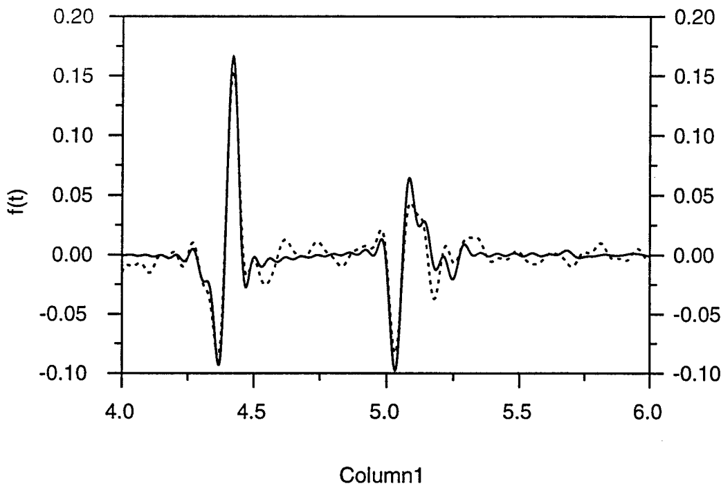
Figure 3.3.1 Comparison of the time domain scattering from the 4", air-filled PVC pipe. The solid line is the theoretical prediction (exact solution for the 2-D TM case) and the dashed line is the laboratory data. The horizontal axis is time in nanosec.
