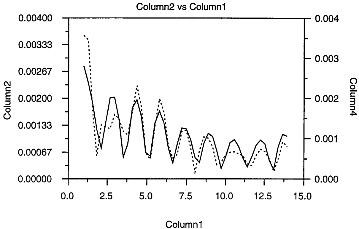
Figure 3.3.2 Frequency comparison of the modulus of the exact solution (solid line) and the laboratory data (dashed line) for the 4" dia., air-filled PVC pipe. The horizontal axis is the frequency in GHz.
