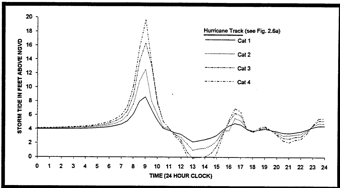
Figure 2.6b Storm tides at Narragansett, Rhode Island for varying hurricane intensity categories.
