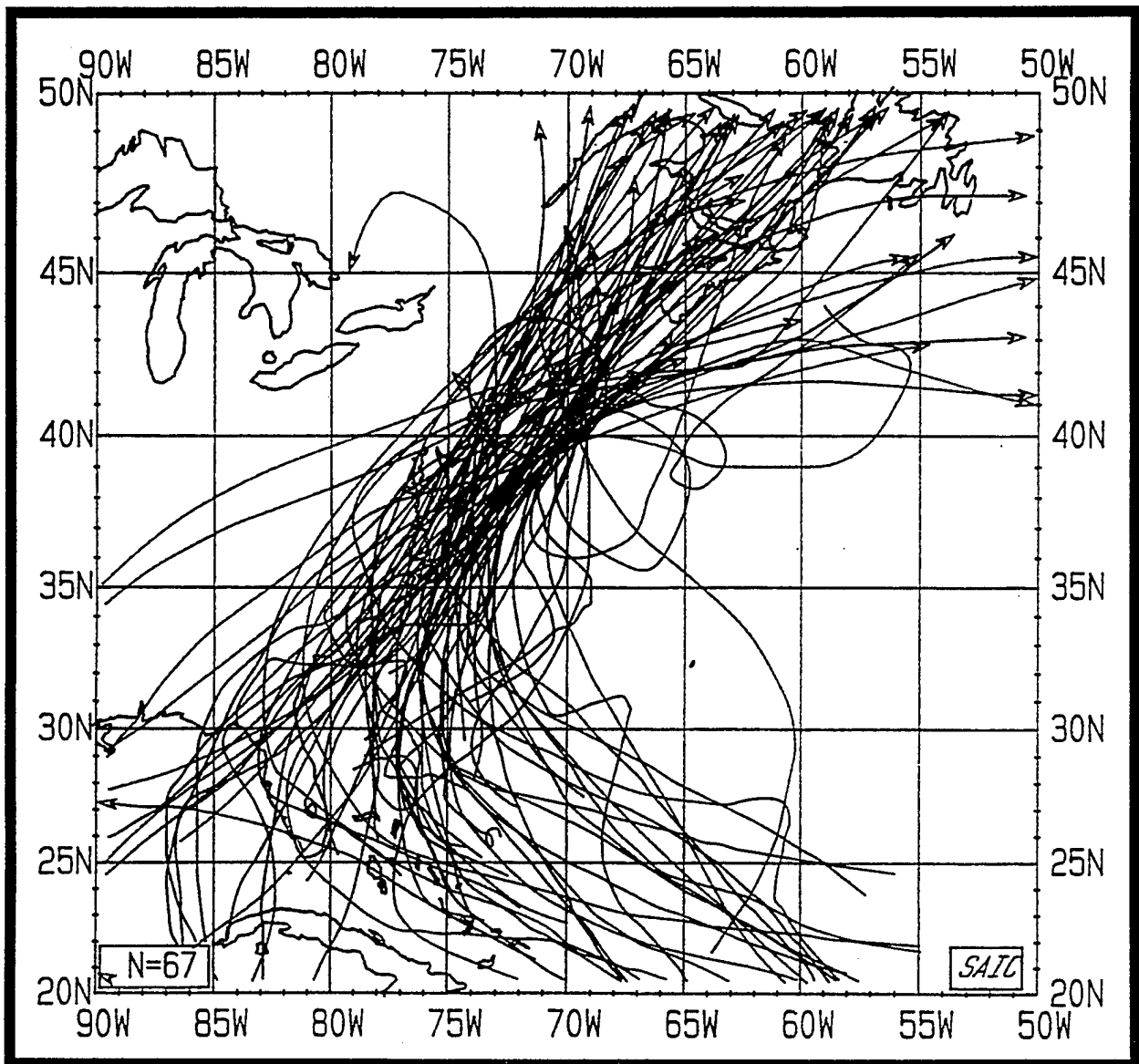
Figure 1.4 Hurricanes and tropical storms passing within 150 statute miles of Newport, Rhode Island from 1886-1993. Source: NHC
