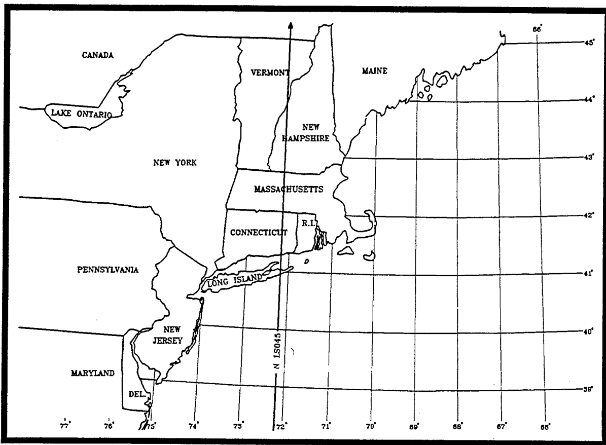
Figure 2.6a Hurricane track for time history data plotted in Fig. 2.6b and Fig. 2.6c.
