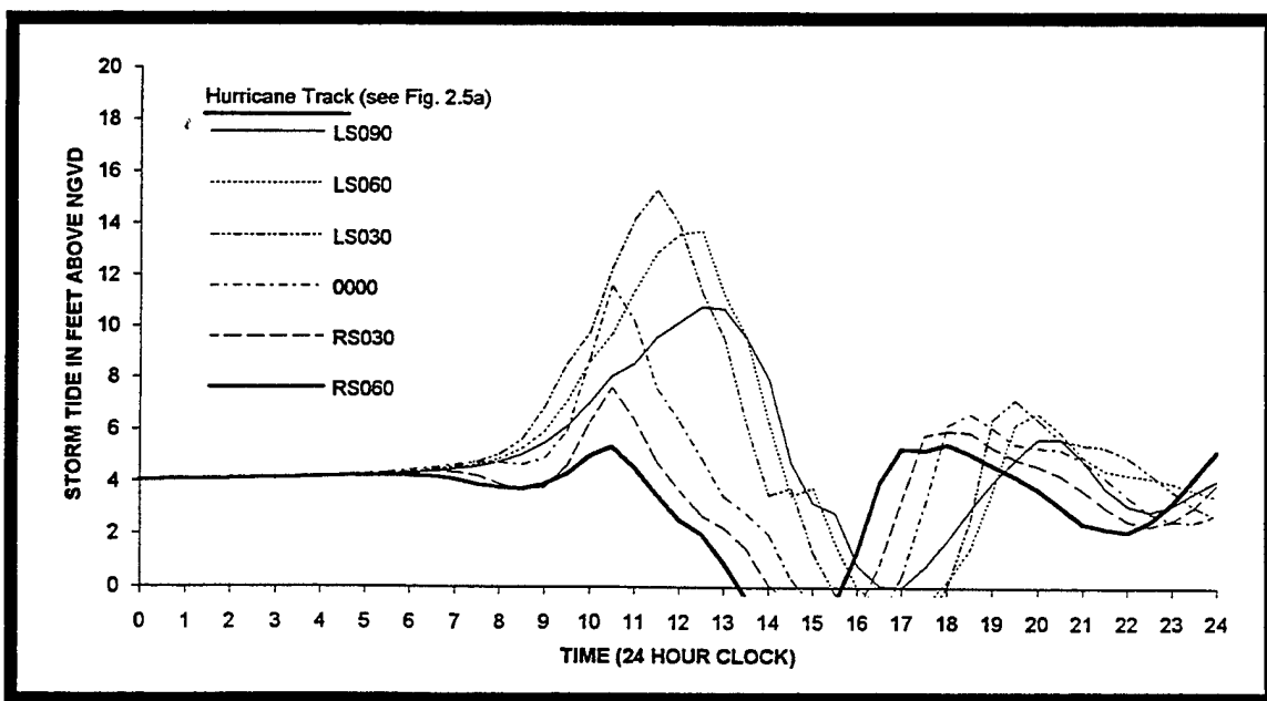
Figure 2.5c Storm tides at Providence, Rhode Island for varying hurricane landfall locations.
