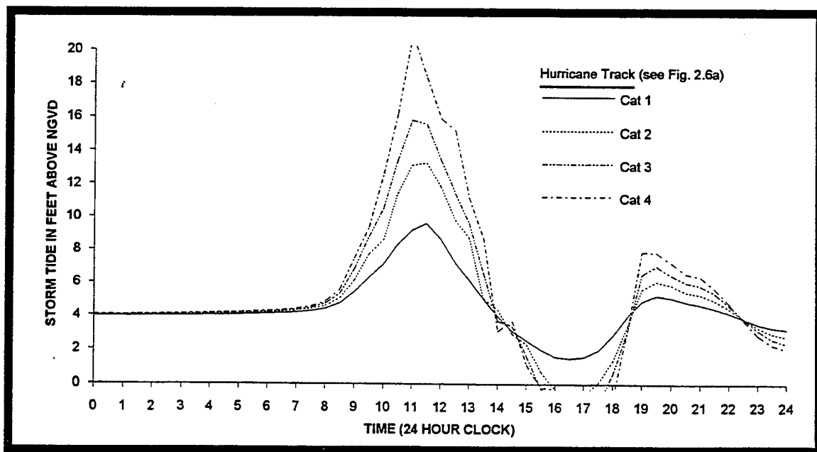
Figure 2.6c Storm tides at Providence, Rhode Island for varying hurricane intensity categories.
