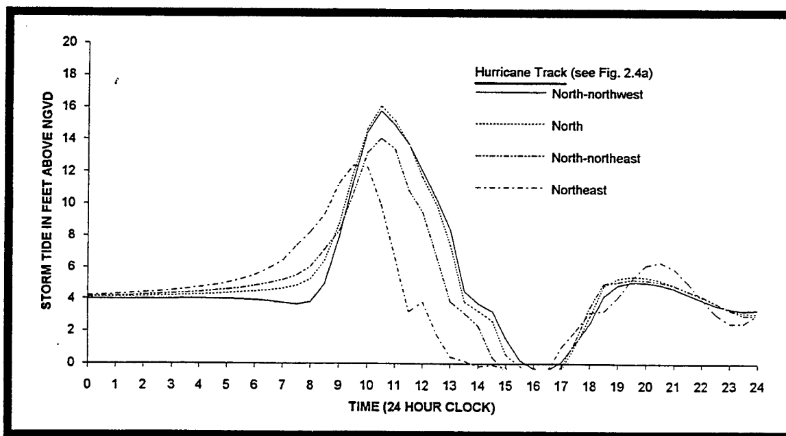
Figure 2.4c Storm tides at Providence, Rhode Island for varying hurricane track directions.
