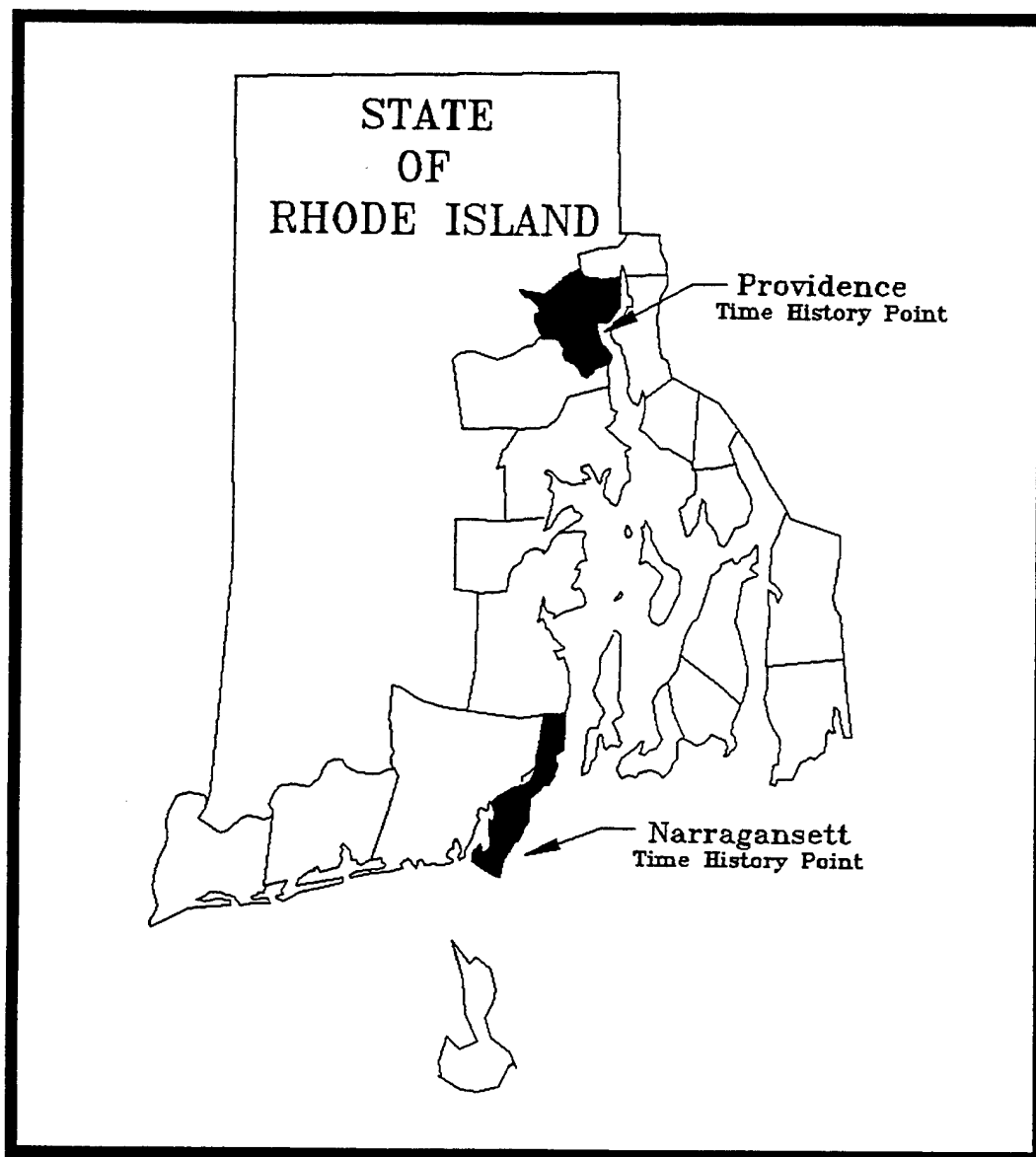
Figure 2.3 Narragansett and Providence, RI Time History Points.
