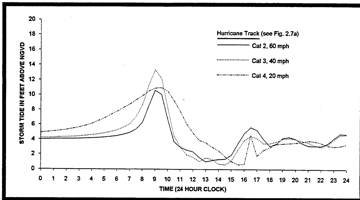
Figure 2.7b Storm tides at Narragansett, Rhode Island for varying hurricane forward speeds.
