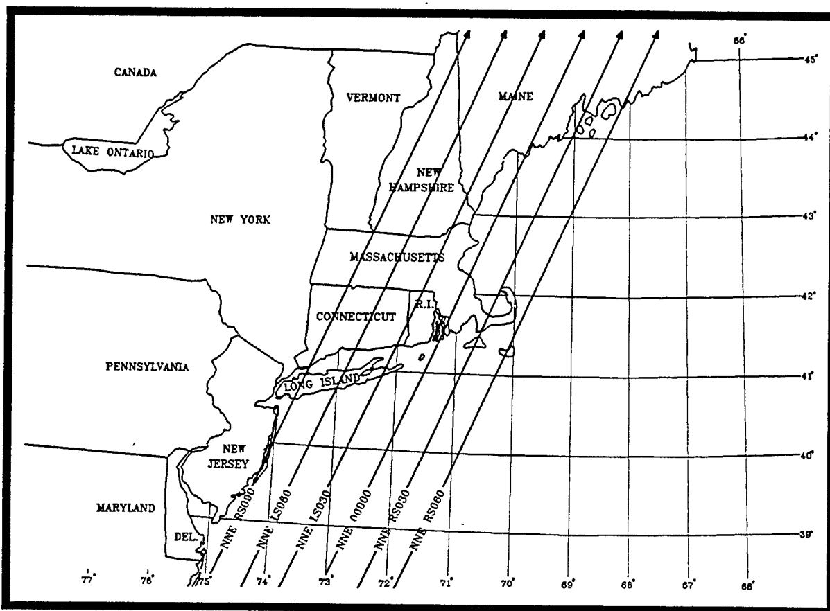
Figure 2.5a Hurricane tracks for time history data plotted in Fig. 2.5b and Fig. 2.5c.
