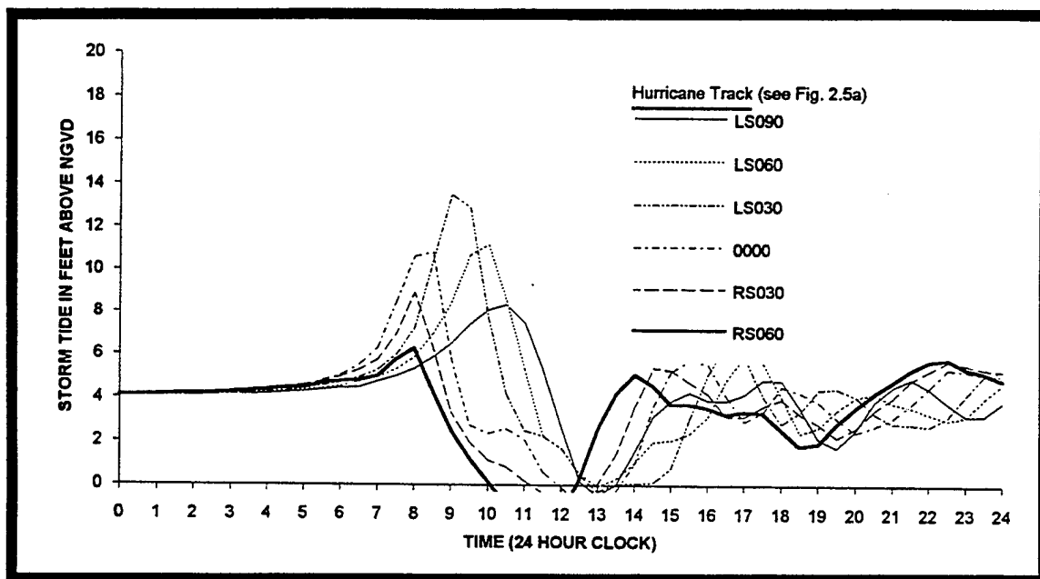
Figure 2.5b Storm tides at Narragansett, Rhode Island for varying hurricane landfall locations.
