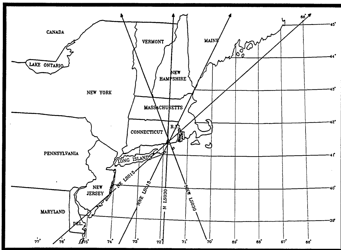
Figure 2.4a Hurricane tracks for time history data plotted in Fig. 2.4b and Fig. 2.4c.
