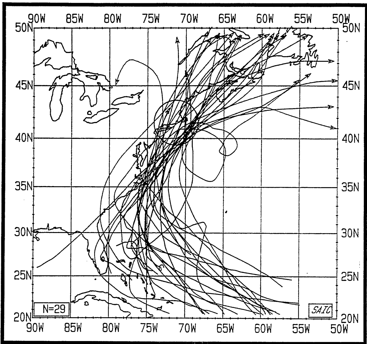
Figure 1.3 Hurricanes passing within 150 statute miles of Newport, Rhode Island from 1886-1993. Source: NHC
