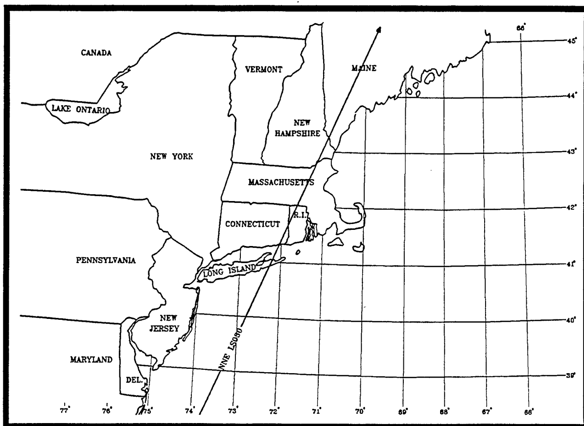
Figure 2.7a Hurricane track for time history data plotted in Fig. 2.7b and Fig. 2.7c.
