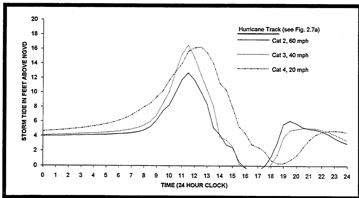
Figure 2.7c Storm tides at Providence, Rhode Island for varying hurricane forward speeds.
