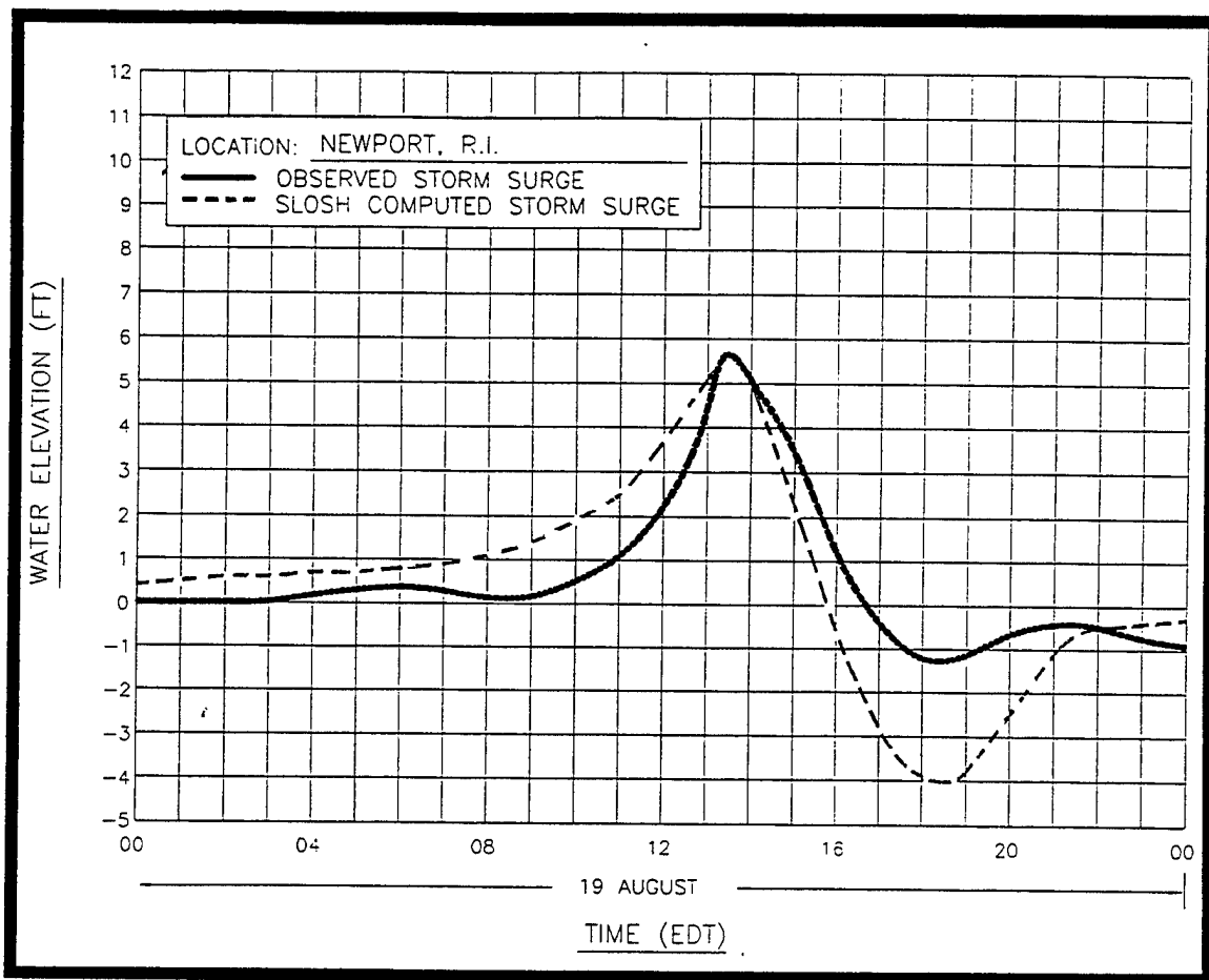
Figure 2.1 Hydrograph at Newport, Rhode Island during the passage of Hurricane Bob on August 19, 1991. Source: NHC
