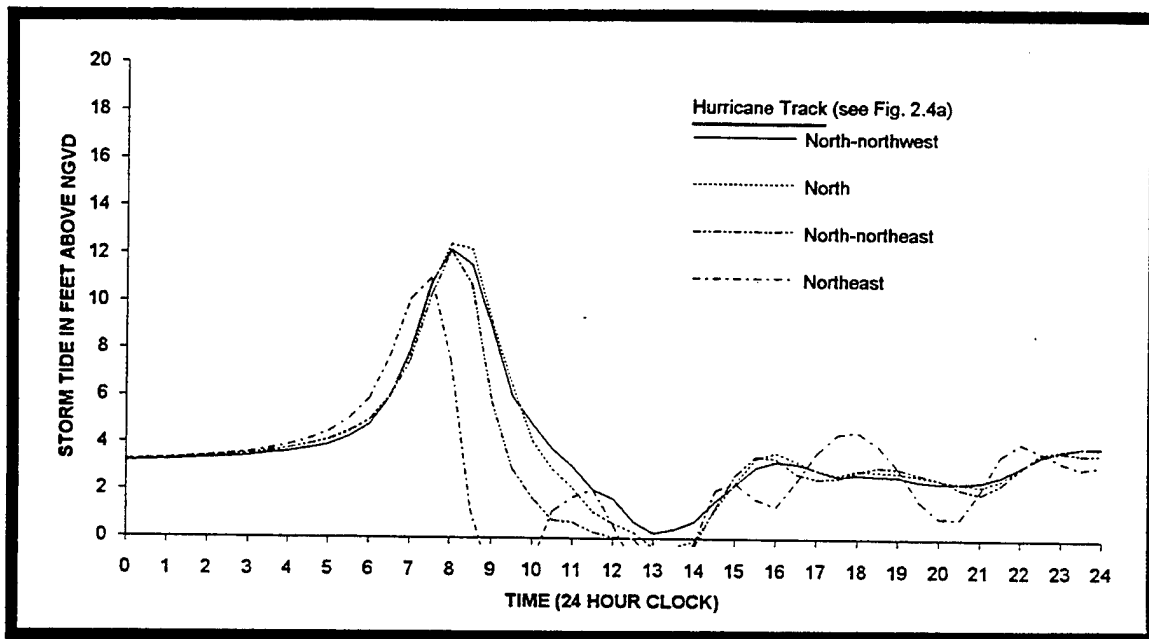
Figure 2.4b Storm tides at Narragansett, Rhode Island for varying hurricane track directions.
