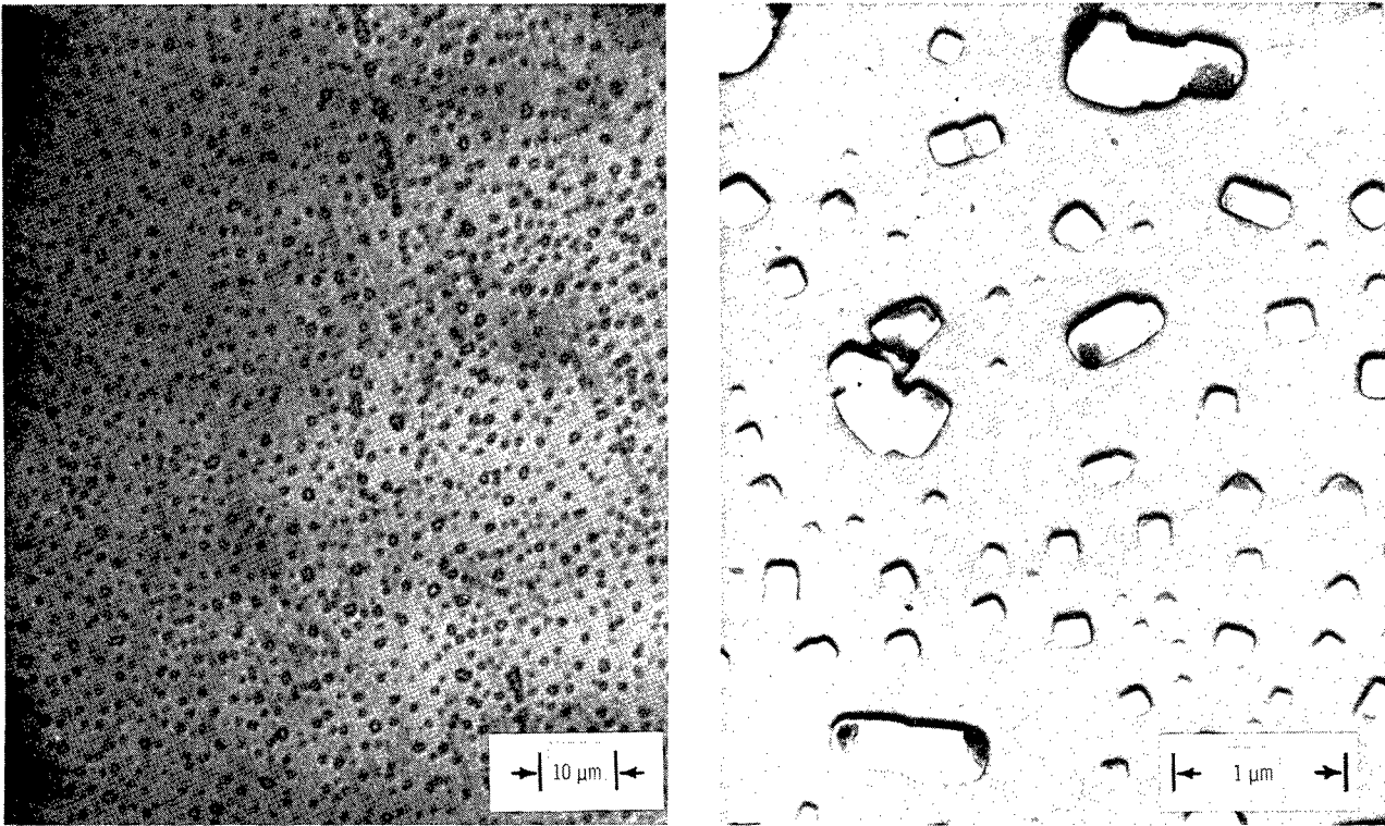
Figure 3. - Salt crystals deposited on hollow titanium alloy specimens at 400° F (205° C).
