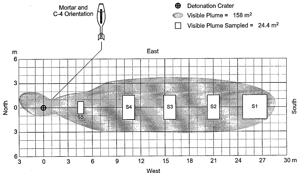
a. First detonation.
