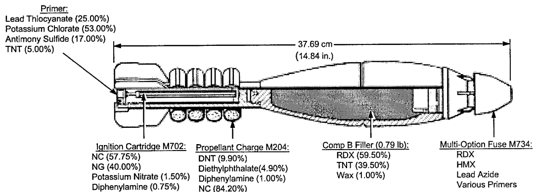
Figure 2. Diagram of 60-mm mortar rounds that were fired at Fort Drum, New York.
