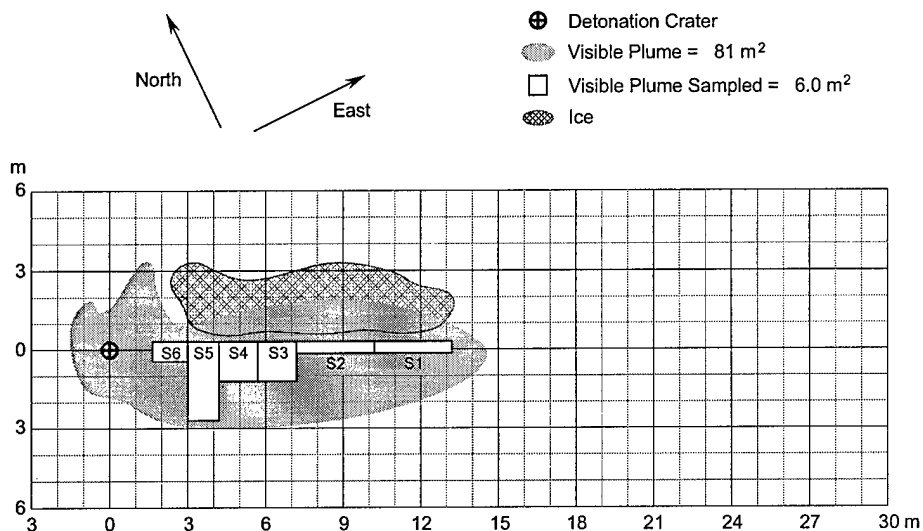
a. First detonation.
