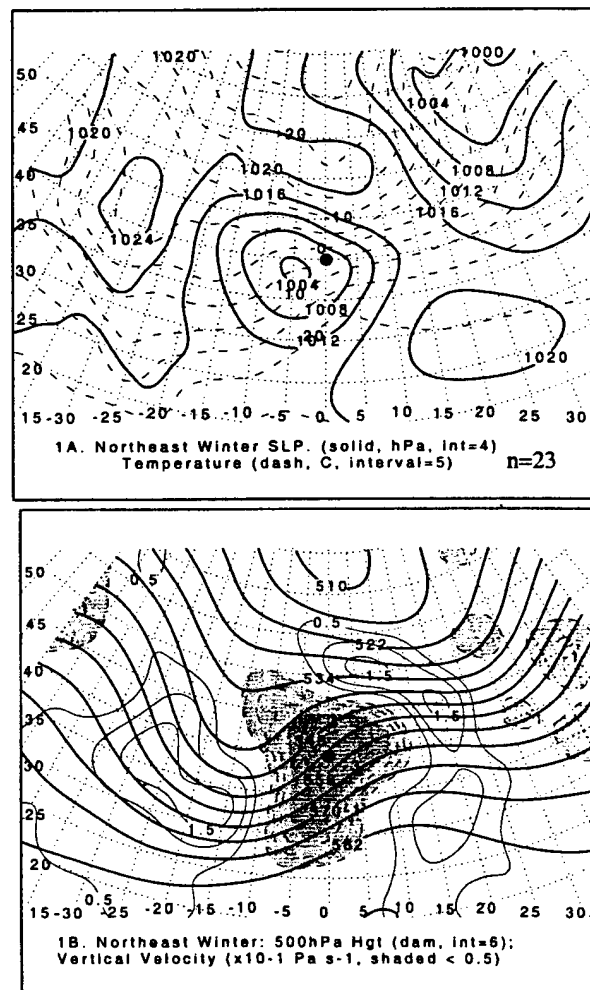
Figure 1. Northeast winter composite. IGW observed at grid center ( 40^\circ\text{N} , 0^\circ\text{W} ): a) Sea level pressure (hPa, solid) and 1000 hPa temperature ( ^\circ\text{C} , dashed), with n indicating the number of IGW events in the composite; b) 500 hPa height (dam, thick solid) and vertical velocity ( 10^{-1} \text{ Pa s}^{-1} , thin solid/dashed, shaded < -0.5 ).
