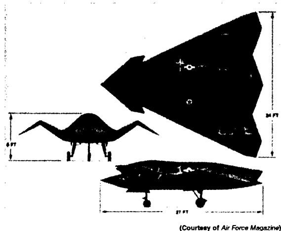
Gull-Wing UCAV with Dimensions—6 Feet Tall, 24 Feet Wide, and 27 Feet Long.
