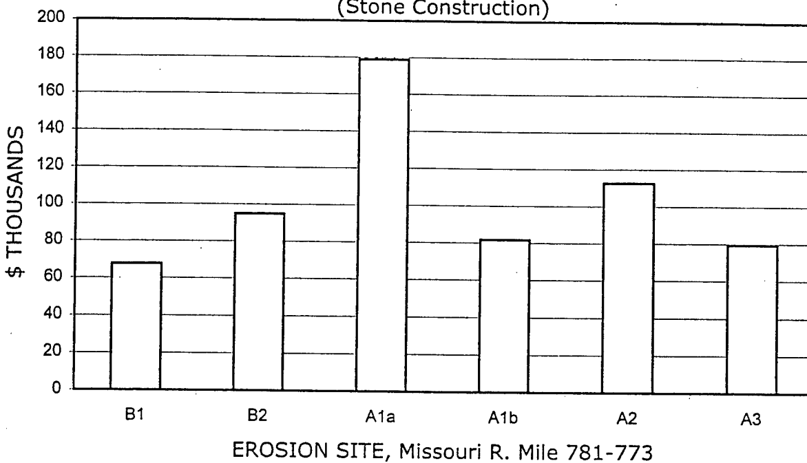
Figure 7 - Estimated Cost Per 1000 Feet of Bank Stabilization (Stone Construction)
