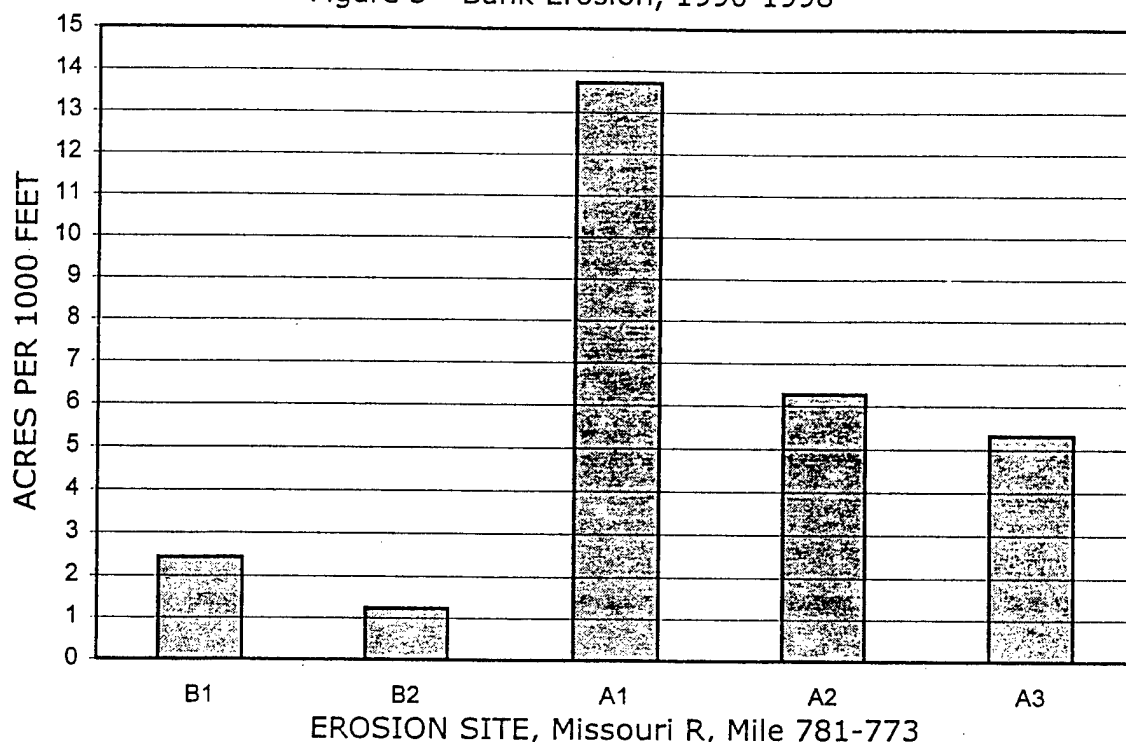
Figure 3 - Bank Erosion, 1990-1998
