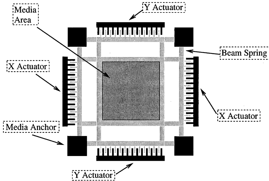
Figure 2: The suspended media sled in the moving media model. The actuators, spring suspension, and the media sled itself are shown. Anchored regions are black and the movable structure is shaded grey.
