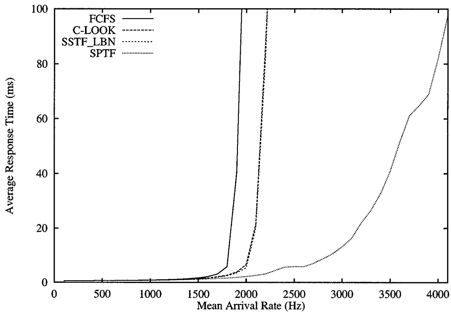
(a) Random (zero time constants) average response time
