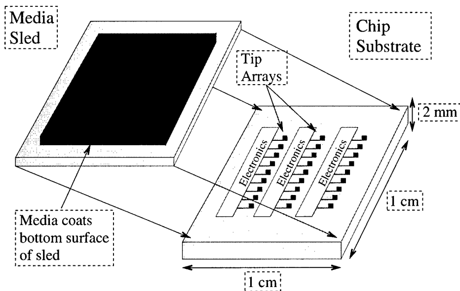
Figure 1: The “moving media” model. The media sled is suspended above the array of fixed tips. The sled moves small distances along the X and Y axes, allowing the fixed tips to address 30–50% of the total media area. This yields capacities of gigabytes per square centimeter.
