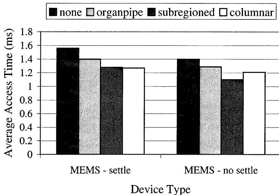
Figure 11: A comparison of various layout schemes for MEMS-based storage devices (§ 5.3). The “MEMS-nosettle” graph shows the same experiment run with zero X settling time. For the default device, the organ pipe, subregioned and columnar layouts achieve a 13–20% performance improvement over the simple layout. It is interesting to note that an optimal disk layout technique does not provide the best performance for MEMS-based storage. Further, for the “no settle” case, the subregioned layout outperforms the others by an additional 20%.
