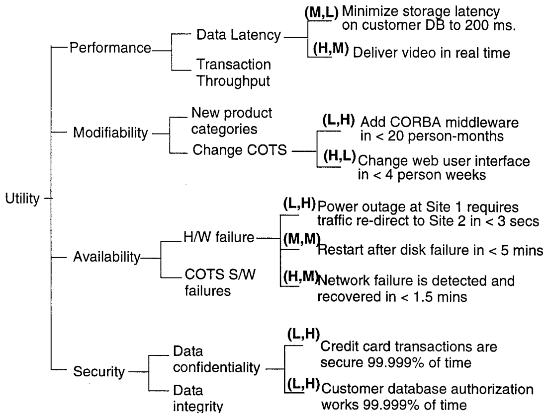
Figure 3: A Sample Utility Tree
