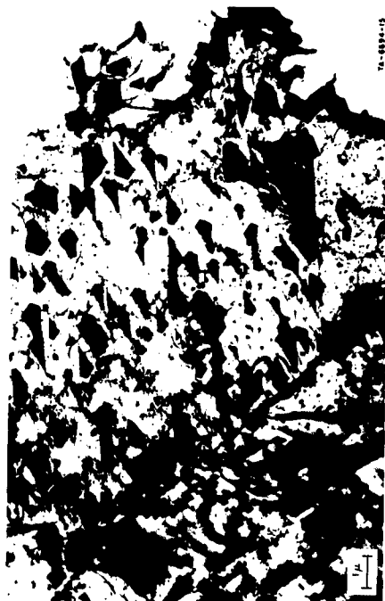
FIG. 15 TRANSMISSION ELECTRON MICROGRAPH OF 304 STAINLESS STEEL FOIL AFTER SIX HOURS EXPOSURE TO LIQUID SODIUM AT 1200°F. Micrograph shows attacked foil edge as well as surface and grain boundary deposit.
