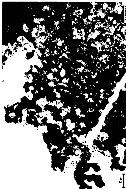
FIG. 8 TRANSMISSION ELECTRON MICROGRAPH OF 304 STAINLESS STEEL FOIL, AFTER ION BOMBARDMENT. The micrograph shows very fine grain structure which resulted from recrystallization due to excessive heating during ion bombardment treatment. Damage to the edge of the foil also occurred during this process.
