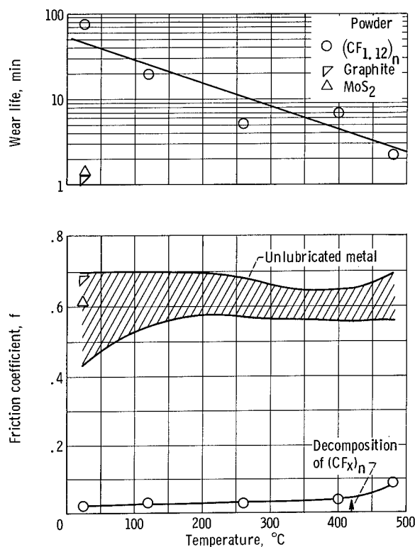
Figure 9. - Effect of temperature on wear life and friction coefficient of graphite fluoride (CF_{1.12})_n , graphite, and molybdenum disulfide powders burnished on glass-peened 301 stainless-steel disks. Riders, 440 C stainless steel; linear sliding speed, 1.6 meters per second; load, 500 grams; atmosphere, dry argon (moisture content, 20 ppm).
