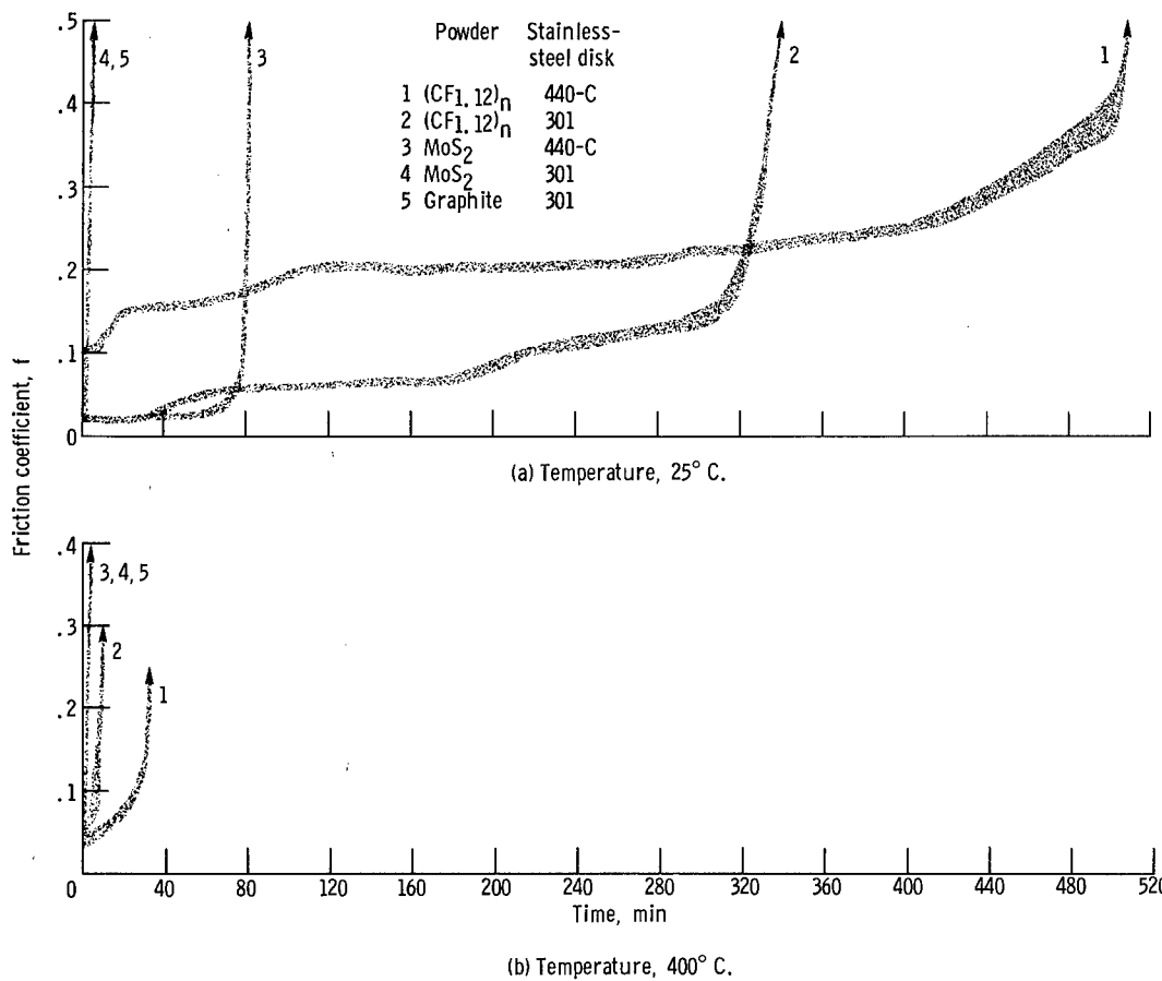
Figure 8. - Variation of friction coefficient with time for burnished films of graphite fluoride ((CF 1.12 ) n ), molybdenum disulfide, and graphite at 25° and 400° C. Riders, 440-C stainless steel; linear sliding speed, 1.6 meters per second; load, 500 grams; atmosphere, dry air (moisture content, 20 ppm).
