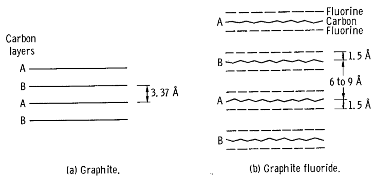
Figure 1. - Structure of graphite and proposed structure of graphite fluoride illustrating expansion of carbon-layer planes due to intercalation of fluorine atoms between them. (Note waviness of carbon planes in graphite fluoride.)
