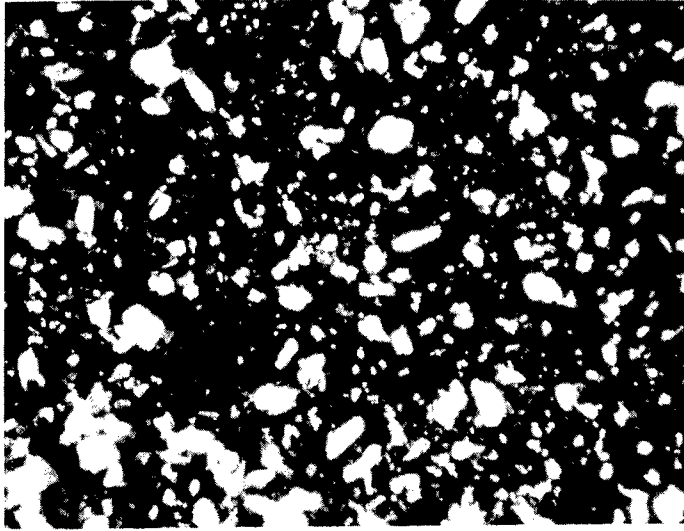
Graphite fluoride
