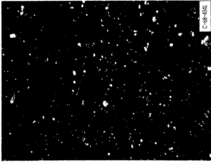
Graphite
