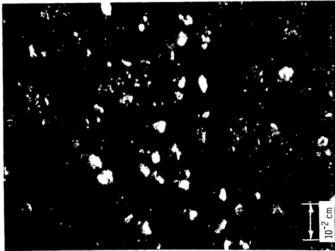
Molybdenum disulfide
