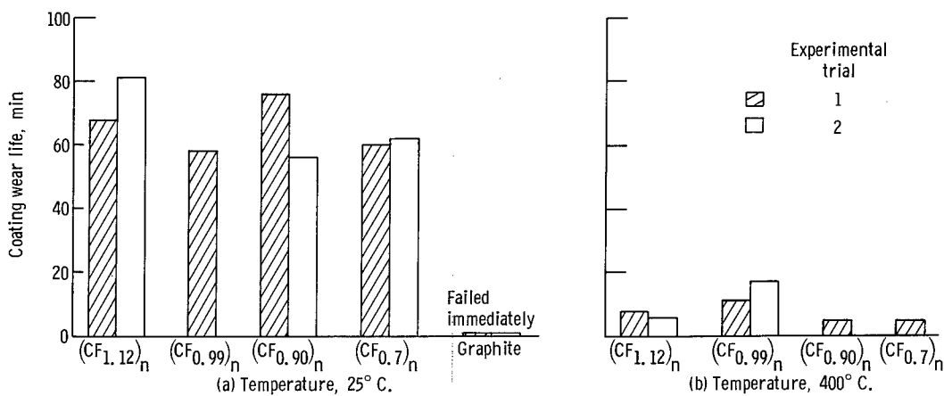
Figure 10. - Effect of fluorine content on wear life of graphite fluoride (CF_x)_n and graphite films burnished on glass-peened 301 stainless-steel disk run at 25° and 400° C. Riders, 440-C stainless steel; linear sliding speed, 1.6 meters per second; load, 500 grams; atmosphere, dry argon (moisture content, 20 ppm).
