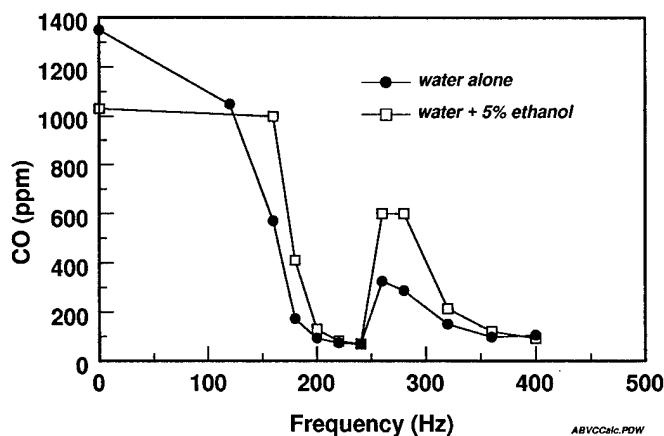
Fig. 13 Effect of organics in the 'surrogate sludge' on performance of the VCC / AB system.
