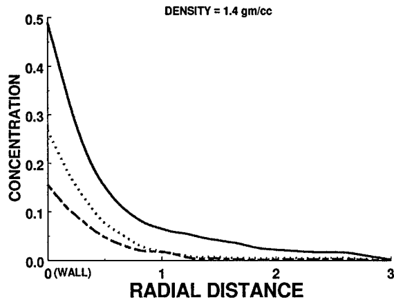
Fig. 8 Radial distribution of particles, measured via laser light scattering, as a function of time after injection. The top curve is a time 0, the second down at 1 minute, and the third at 2 minutes. The horizontal axis is inches. The dry milk particles were sieved to around 60 \mu\text{m} or below.
