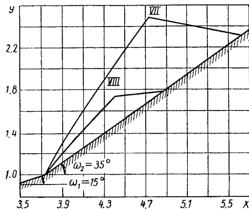
FIGURE 4. Compression shock and boundary characteristic for M_{in} = 2.594 (VII) and M_{in} = 4.097 (VIII); \omega_1 = 15^\circ , \omega_2 = 35^\circ
