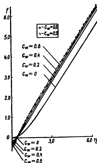
FIGURE 3. Function f vs. \eta for various c values at the wall
