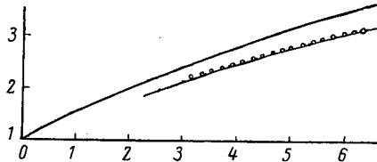
FIGURE 7. Jet boundary and shock for M_0=3.0 , M_b=5.2867 . The dash-dot line gives a shock whose origin is defined as the intersection point of the boundary characteristic of the fan with the first characteristic reflected from the jet boundary; circles mark the results obtained with the intersection of the fifth reflected characteristic
