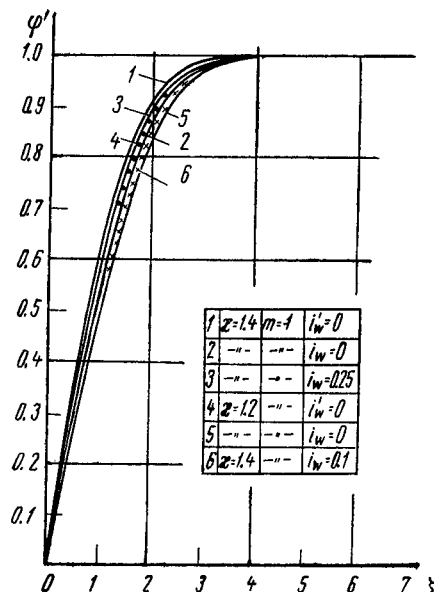
FIGURE 2. Velocity profiles u=\varphi'(\zeta) in boundary layer with \beta=0
