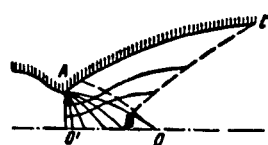
FIGURE 1. Axisymmetric nozzle with an angular point
