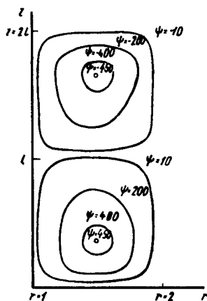
FIGURE 3. \Psi -field for H=2l (flow II) at time t=30; \tau = \frac{1}{32}
