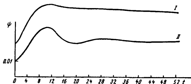
FIGURE 1. Variation of \Psi in time:
