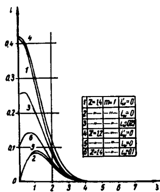
FIGURE 1. Enthalpy i vs. \zeta = \frac{\sqrt{R} \cdot \eta}{2M\sqrt{\xi}} ( \eta , \xi are the Dorodnitsyn variables) in boundary layer with \beta=0
