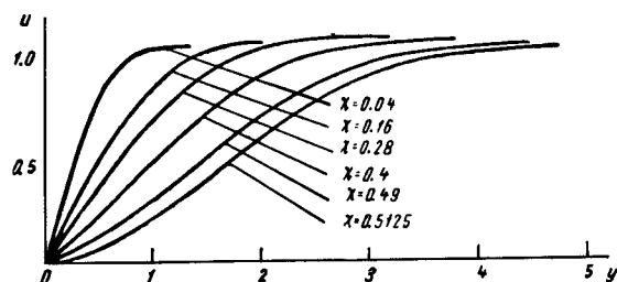
FIGURE 1. Velocity profiles u for a = 0.008
