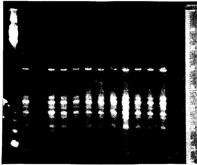
Figure 1. PCR products after primary amplification of genomic DNAs from four shovelnose, four pallids, and four hybrid sturgeons. Lane 1, BRL 123 bp DNA ladder. Lanes 2-5, ST 194-197 (shovelnose). Lanes 6-9, ST 74, 109-111 (pallid). Lanes 10-13, ST 77-80 (hybrids).
