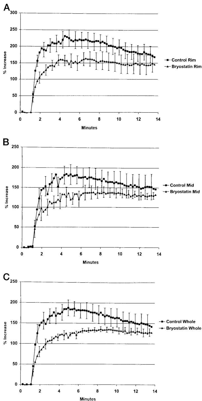
Fig. 4 Percent change in tumor signal intensity after a dose of Gd-DTPA in control tumor-bearing mice or 12 h after the tumor-bearing mice were treated with bryostatin-1. A, rim of tumor; B, central core of tumor; C, whole tumor. There were modest differences in the center and rim of the tumor between control and tumor-bearing mice treated with bryostatin-1, which approached significance. The change in maximum enhancement over the whole tumor was significant ( P = 0.05 ).
