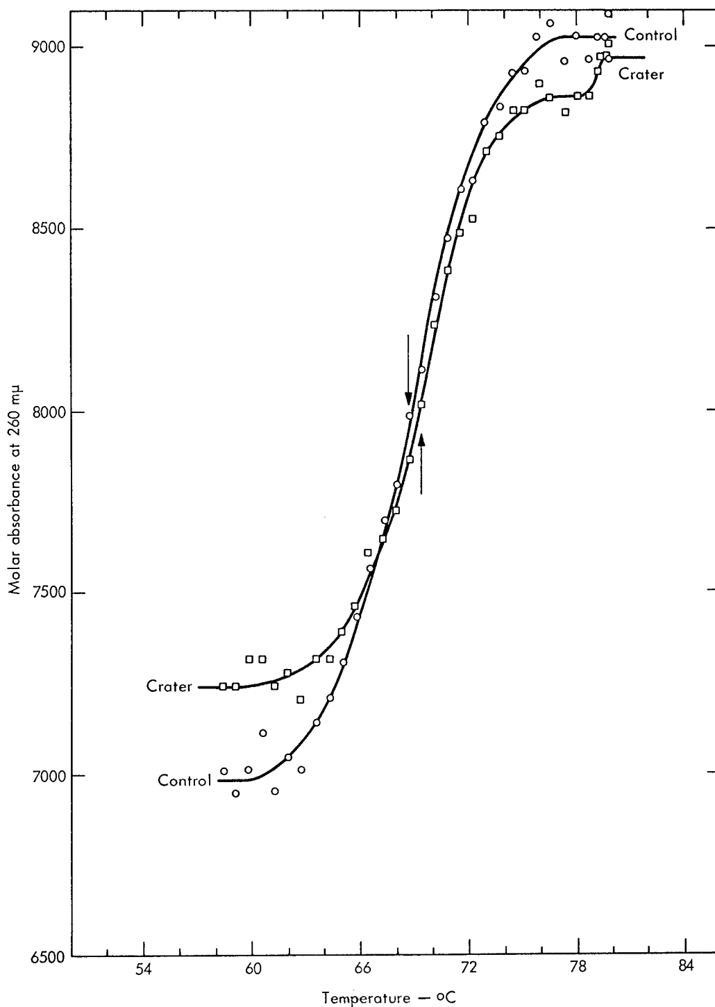
Fig. 4. Thermal transition of ultraviolet absorbance at 260 \mu . Data on the ordinate are expressed in terms of molar absorbance based upon the concentration of the solution as determined from analysis of the ultraviolet spectrum after denaturation. 23 The molar absorbance of crater DNA is higher than that of control DNA before heating whereas the values are nearly equal after heating. Expression of the ordinate values in terms of relative absorbance, as is conventional for thermal transition curves, would lead to misinterpretation of these data. The arrows point to the T_m values. Note the small second transition T_m' at about 80°C exhibited by crater DNA.
