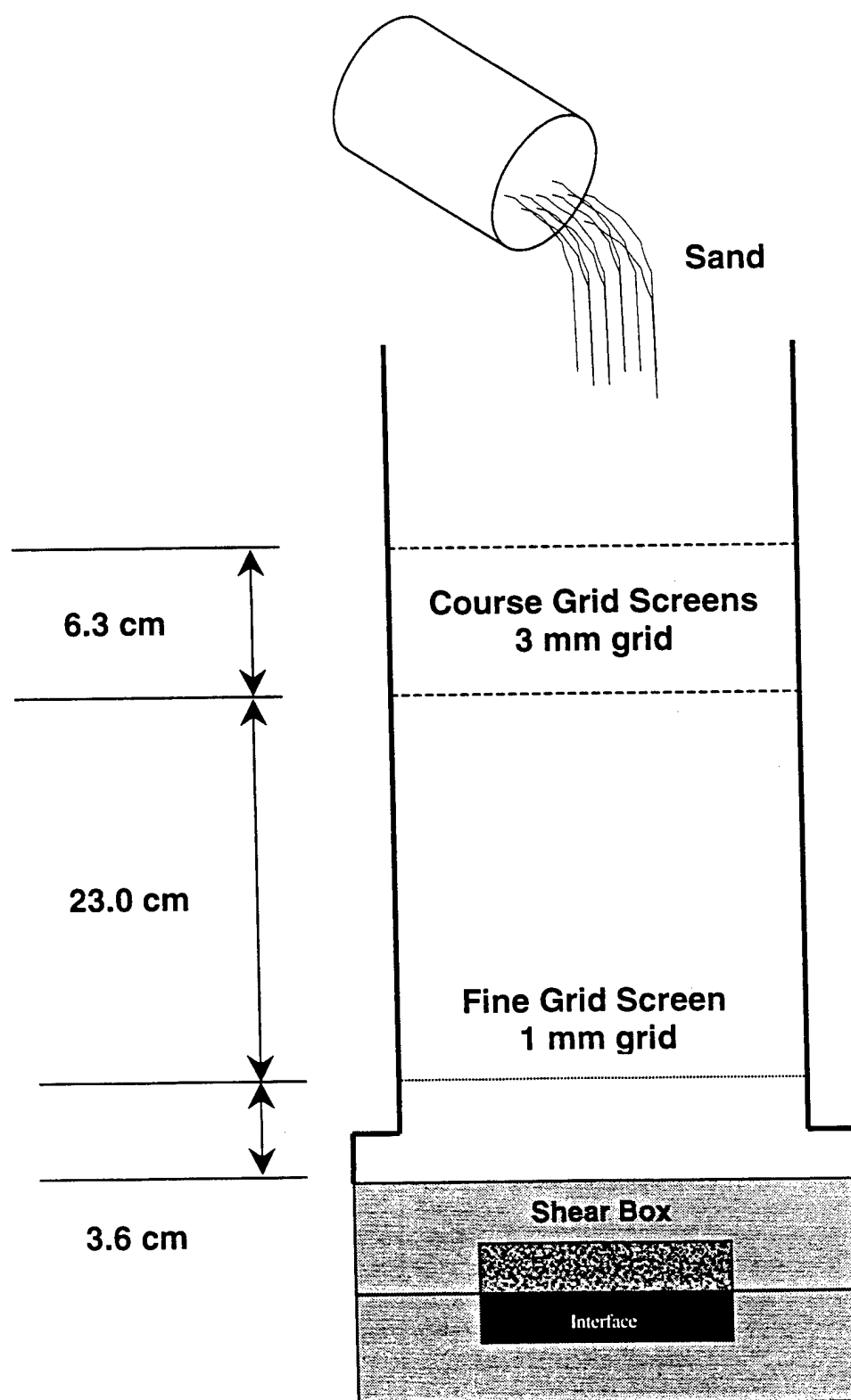
Figure 2-7 Diagram of Rain-Through Air Sample Preparation Device
