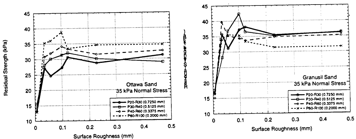
Figure 2-24 Residual Strength
