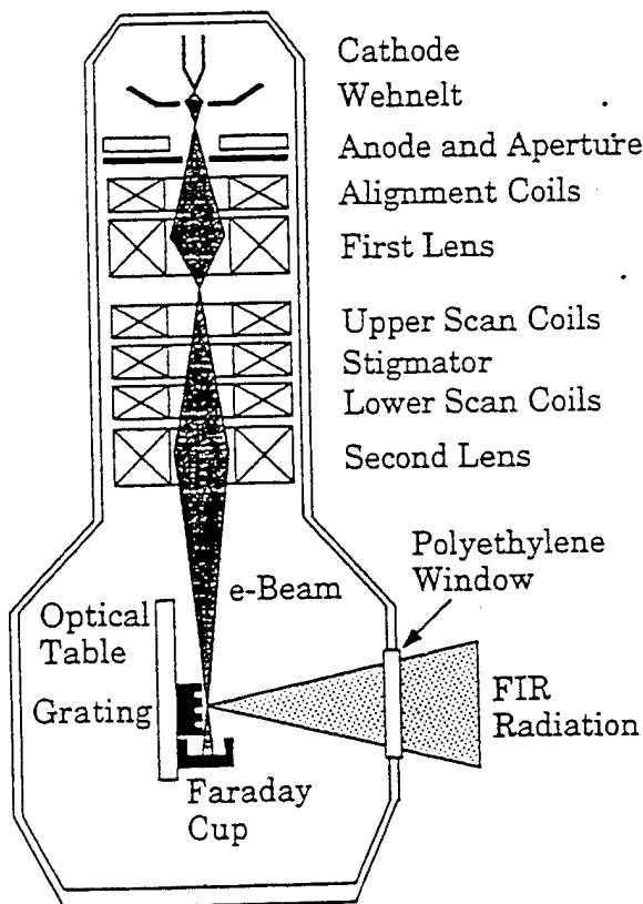
FIG. 1. Diagram of the SEM optical system.
