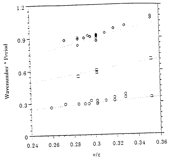
Fig. 6. Measured wave numbers in units of the grating period(s) versus relative beam velocity. Three orders are shown.
